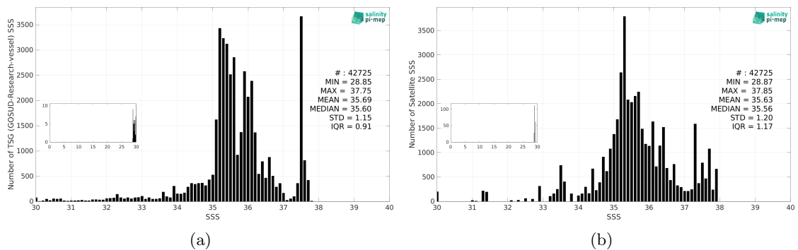
Figure 3: Histograms of SSS from TSG (GOSUD-Research-vessel) (a) and Aquarius SSS L2 OR v5 (NASA-GSFC) (b) considering all match-up pairs per bins of 0.1 over the Amazon and Orinoco river plumes Pi-MEP region and for the full satellite product period.
