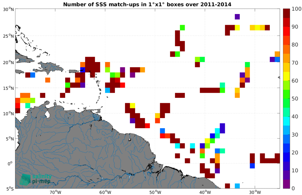
Figure 5: Number of SSS match-ups between TSG (GOSUD-Research-vessel) SSS and the Aquarius SSS L2 OR v5 (NASA-GSFC) SSS product for the Amazon and Orinoco river plumes Pi-MEP region over 1^\circ \times 1^\circ boxes and for the full satellite product period.
