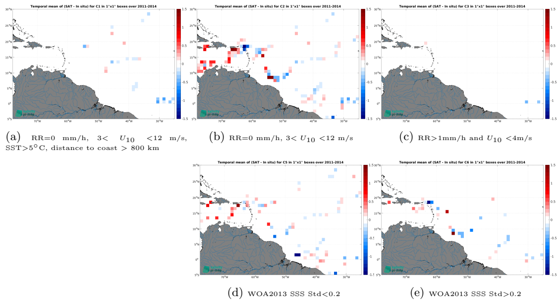
Figure 14: Temporal mean gridded over spatial boxes of size 1^\circ \times 1^\circ of \Delta SSS (Aquarius SSS L2 OR v5 (NASA-GSFC) - TSG (GOSUD-Research-vessel)) for 5 different subdatasets corresponding to:RR=0 mm/h, 3 < U_{10} < 12 m/s, SST>5°C, distance to coast > 800 km (a), RR=0 mm/h, 3 < U_{10} < 12 m/s (b), RR>1mm/h and U_{10} < 4 m/s (c), WOA2013 SSS Std<0.2 (d), WOA2013 SSS Std>0.2 (e).
