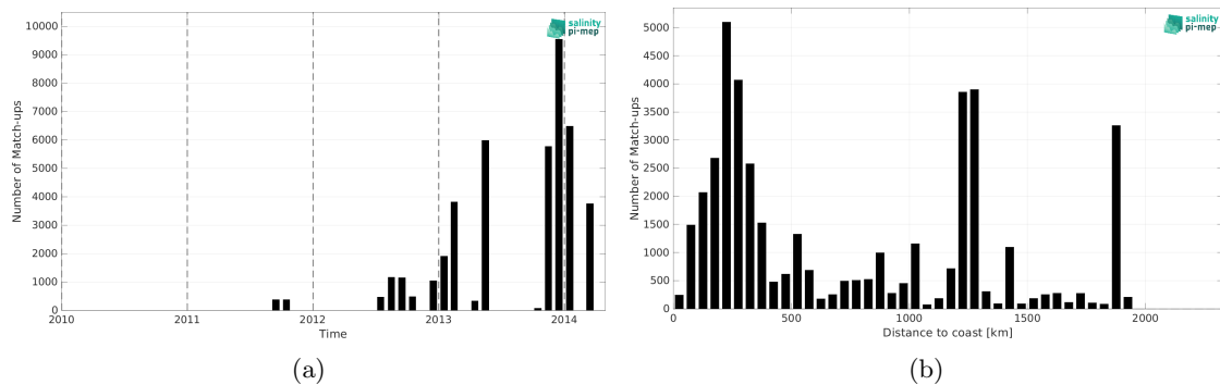
Figure 2: Number of match-ups between TSG (GOSUD-Research-vessel) and Aquarius SSS L2 OR v5 (NASA-GSFC) SSS as a function of time (a) and as function of the distance to coast (b) over the Amazon and Orinoco river plumes Pi-MEP region and for the full satellite product period.
