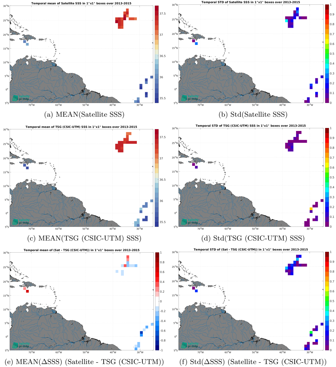
Figure 7: Temporal mean (left) and Std (right) of SSS from Aquarius SSS L2 OR v5 (NASA-GSFC) (top), TSG (CSIC-UTM) (middle), and of \Delta SSS (Satellite - TSG (CSIC-UTM)). Only match-up pairs are used to generate these maps.
