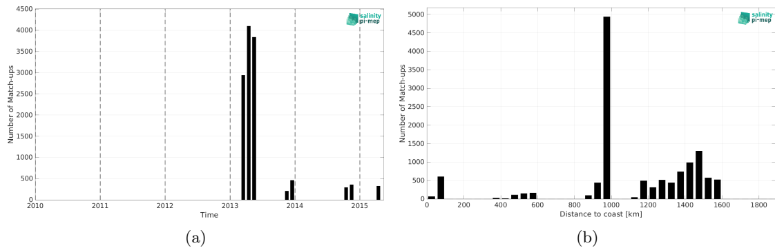
Figure 2: Number of match-ups between TSG (CSIC-UTM) and Aquarius SSS L2 OR v5 (NASA-GSFC) SSS as a function of time (a) and as function of the distance to coast (b) over the Amazon and Orinoco river plumes Pi-MEP region and for the full satellite product period.
