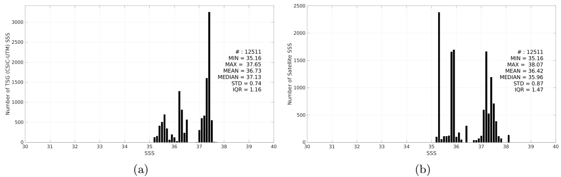
Figure 3: Histograms of SSS from TSG (CSIC-UTM) (a) and Aquarius SSS L2 OR v5 (NASA-GSFC) (b) considering all match-up pairs per bins of 0.1 over the Amazon and Orinoco river plumes Pi-MEP region and for the full satellite product period.
