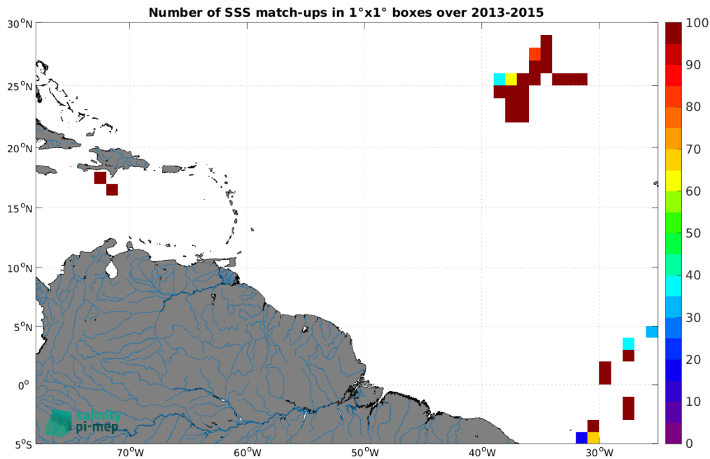
Figure 5: Number of SSS match-ups between TSG (CSIC-UTM) SSS and the Aquarius SSS L2 OR v5 (NASA-GSFC) SSS product for the Amazon and Orinoco river plumes Pi-MEP region over 1^\circ \times 1^\circ boxes and for the full satellite product period.
