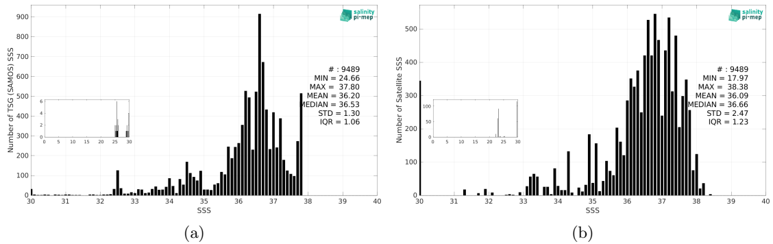
Figure 3: Histograms of SSS from TSG (SAMOS) (a) and Aquarius SSS L2 CAP v5 (JPL) (b) considering all match-up pairs per bins of 0.1 over the Amazon and Orinoco river plumes Pi-MEP region and for the full satellite product period.
