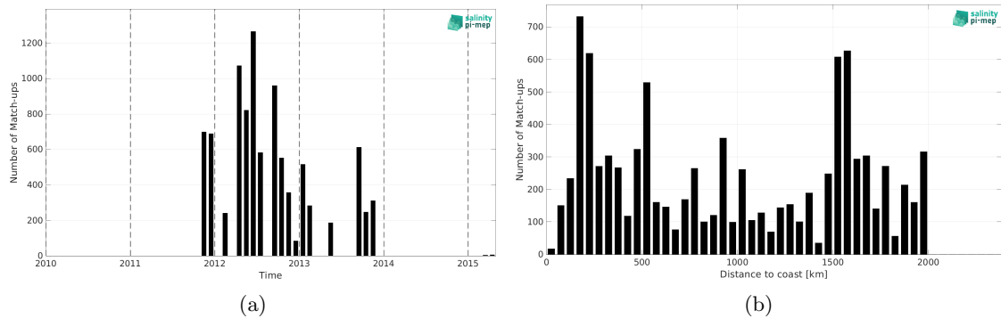
Figure 2: Number of match-ups between TSG (SAMOS) and Aquarius SSS L2 CAP v5 (JPL) SSS as a function of time (a) and as function of the distance to coast (b) over the Amazon and Orinoco river plumes Pi-MEP region and for the full satellite product period.
