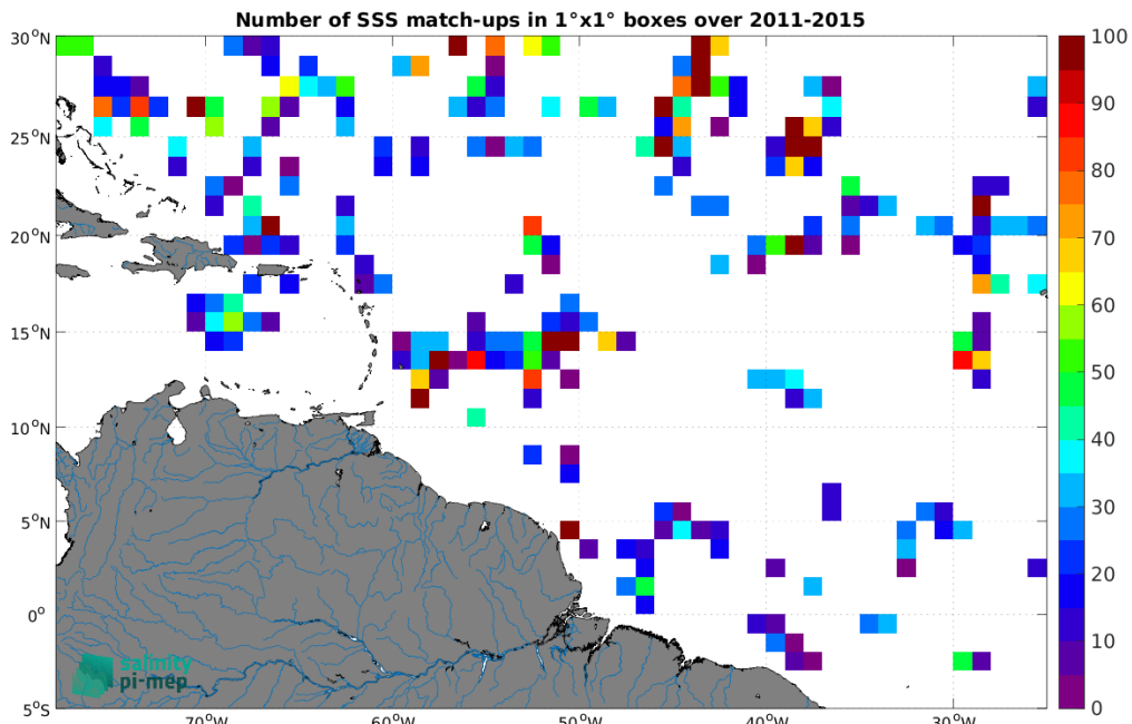
Figure 5: Number of SSS match-ups between TSG (SAMOS) SSS and the Aquarius SSS L2 CAP v5 (JPL) SSS product for the Amazon and Orinoco river plumes Pi-MEP region over 1^\circ \times 1^\circ boxes and for the full satellite product period.
