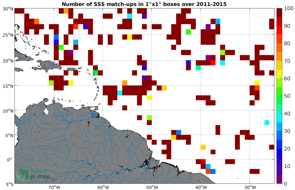
Figure 4: Number of SSS match-ups between TSG (SAMOS) SSS and the Aquarius SSS L2 CAP v5 (JPL) SSS product for the Amazon and Orinoco river plumes Pi-MEP region over 1^{\circ} \times 1^{\circ} boxes and for the full satellite product period.
