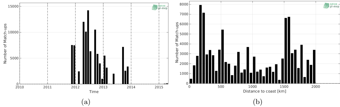
Figure 1: Number of match-ups between TSG-SAMOS and Aquarius-L2-JPL-V5 SSS as a function of time (a) and as function of the distance to coast (b) over the Amazon and Orinoco river plumes Pi-MEP region and for the full satellite product period.
