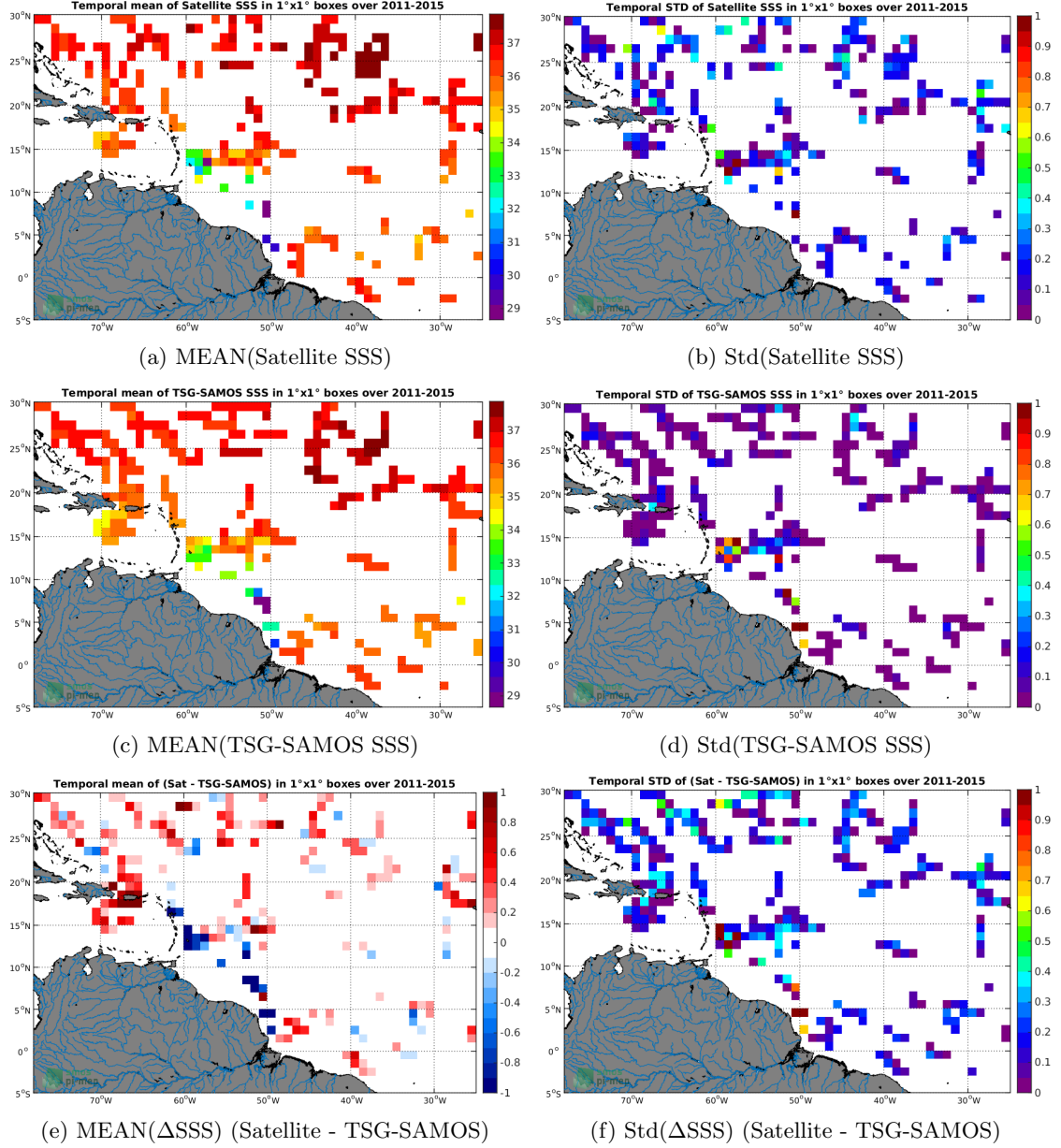
Figure 6: Temporal mean (left) and Std (right) of SSS from Aquarius-L2-JPL-V5 (top), TSG-SAMOS (middle), and of \Delta SSS (Satellite - TSG-SAMOS). Only match-up pairs are used to generate these maps.
