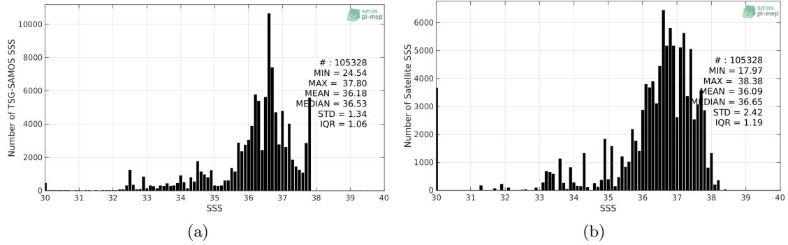
Figure 2: Histograms of SSS from TSG-SAMOS (a) and Aquarius-L2-JPL-V5 (b) considering all match-up pairs per bins of 0.1 over the Amazon and Orinoco river plumes Pi-MEP region and for the full satellite product period.
