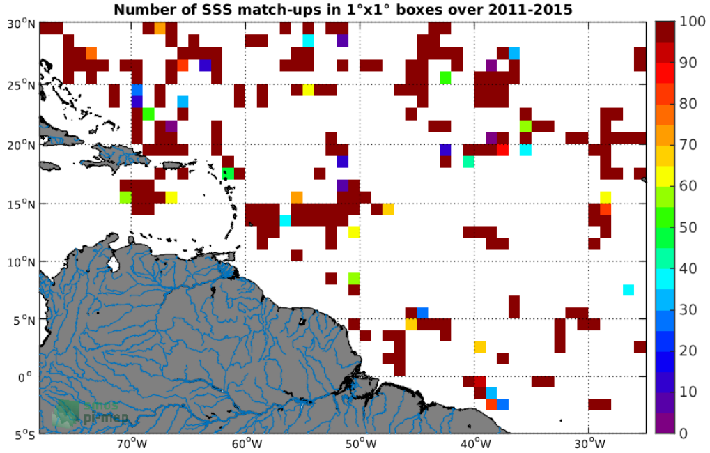
Figure 4: Number of SSS match-ups between TSG-SAMOS SSS and the Aquarius-L2-JPL-V5 SSS product for the Amazon and Orinoco river plumes Pi-MEP region over 1^\circ \times 1^\circ boxes and for the full satellite product period.
