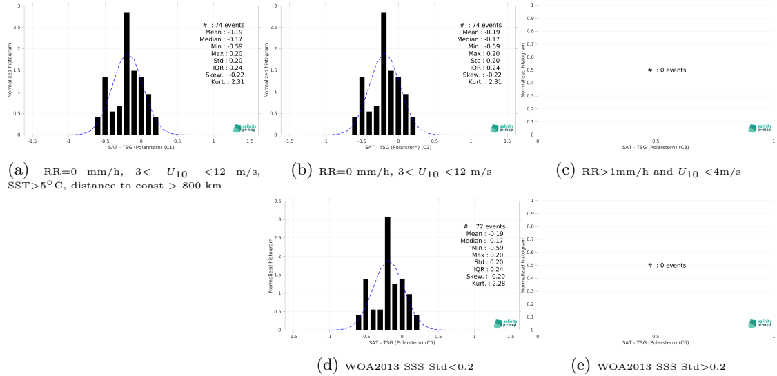
Figure 15: Normalized histogram of \Delta SSS (Aquarius SSS L2 CAP v5 (JPL) - TSG (Polarstern)) for 5 different subdatasets corresponding to: RR=0 mm/h, 3 < U_{10} < 12 m/s, SST>5°C, distance to coast > 800 km (a), RR=0 mm/h, 3 < U_{10} < 12 m/s (b), RR>1mm/h and U_{10} < 4 m/s (c), WOA2013 SSS Std<0.2 (d), WOA2013 SSS Std>0.2 (e).
