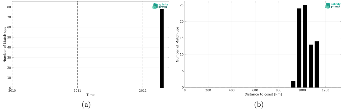
Figure 2: Number of match-ups between TSG (Polarstern) and Aquarius SSS L2 CAP v5 (JPL) SSS as a function of time (a) and as function of the distance to coast (b) over the Amazon and Orinoco river plumes Pi-MEP region and for the full satellite product period.
