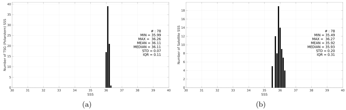
Figure 3: Histograms of SSS from TSG (Polarstern) (a) and Aquarius SSS L2 CAP v5 (JPL) (b) considering all match-up pairs per bins of 0.1 over the Amazon and Orinoco river plumes Pi-MEP region and for the full satellite product period.
