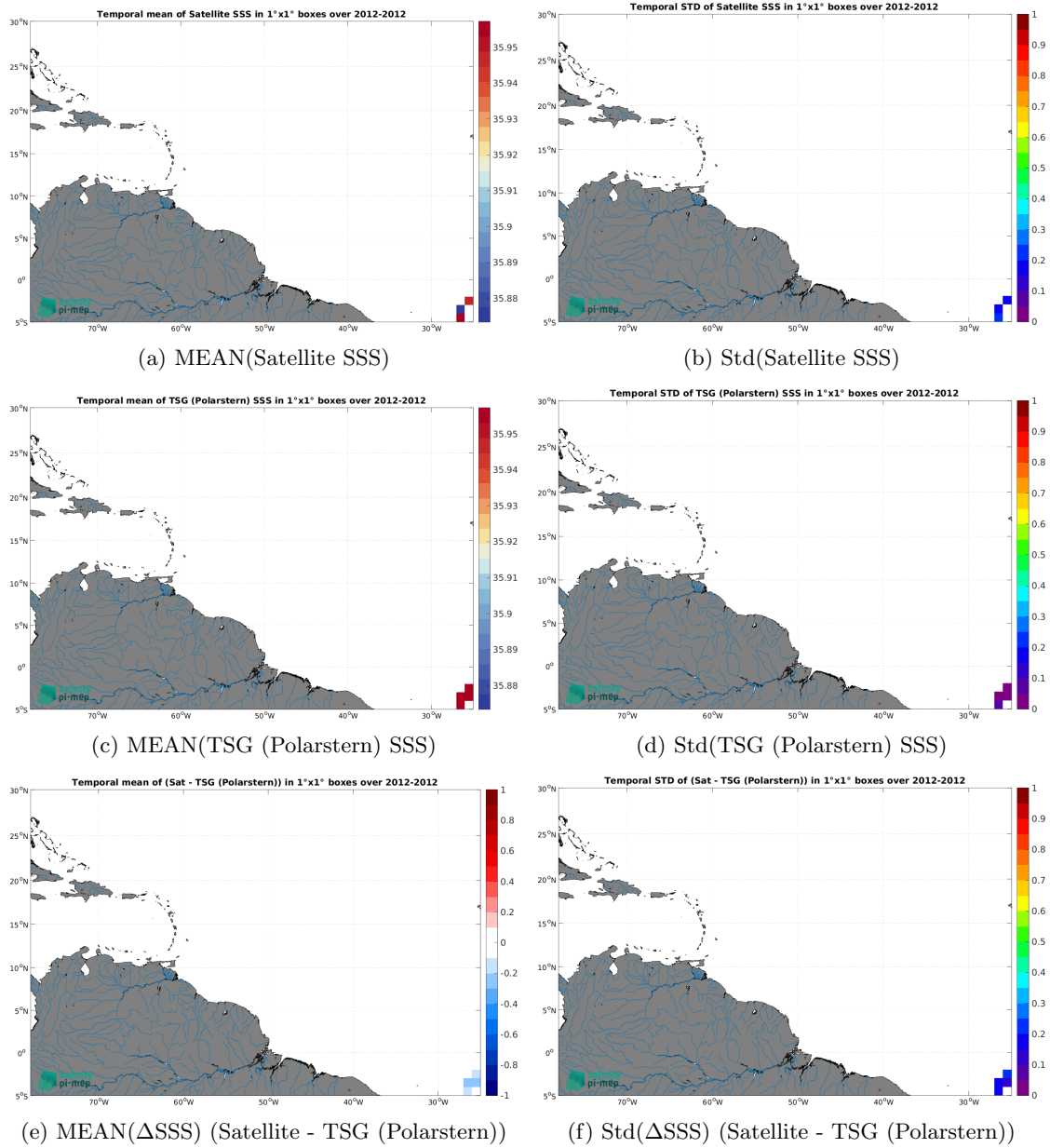
Figure 7: Temporal mean (left) and Std (right) of SSS from Aquarius SSS L2 CAP v5 (JPL) (top), TSG (Polarstern) (middle), and of \Delta SSS (Satellite - TSG (Polarstern)). Only match-up pairs are used to generate these maps.
