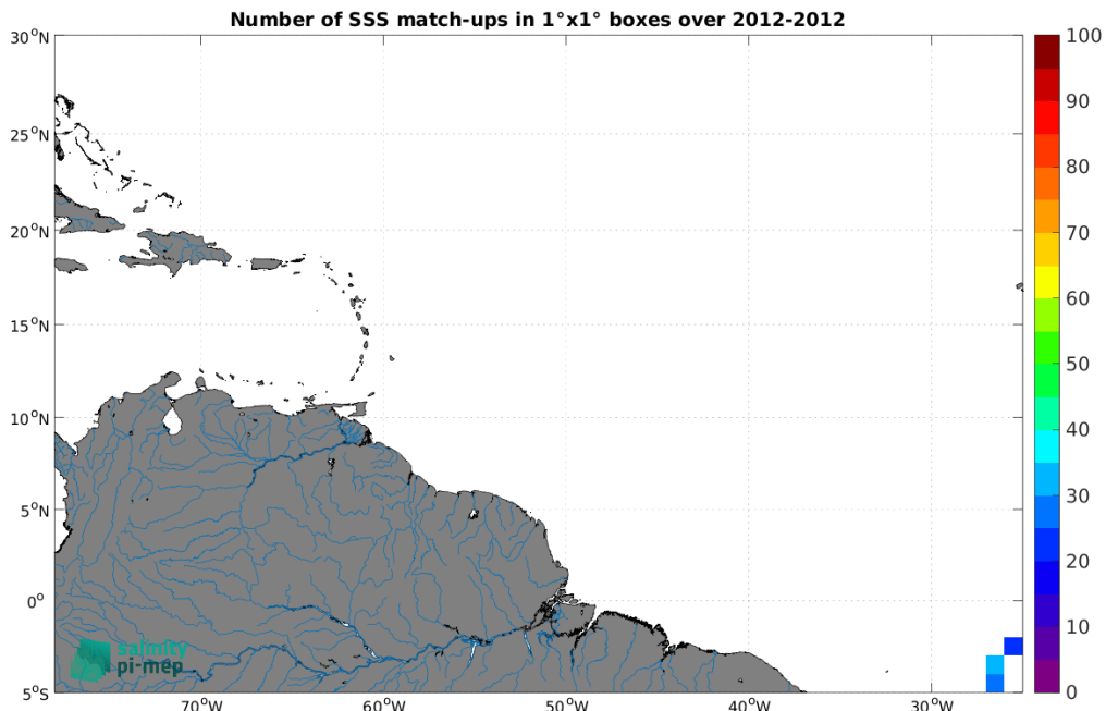
Figure 5: Number of SSS match-ups between TSG (Polarstern) SSS and the Aquarius SSS L2 CAP v5 (JPL) SSS product for the Amazon and Orinoco river plumes Pi-MEP region over 1^\circ \times 1^\circ boxes and for the full satellite product period.
