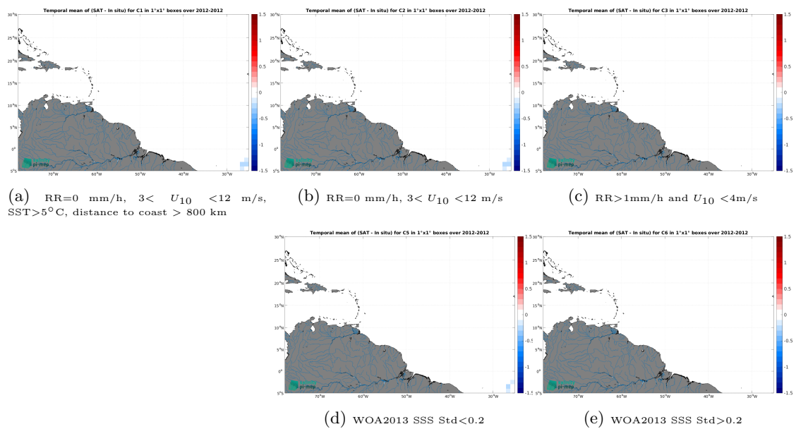
Figure 14: Temporal mean gridded over spatial boxes of size 1^\circ \times 1^\circ of \Delta SSS (Aquarius SSS L2 CAP v5 (JPL) - TSG (Polarstern)) for 5 different subdatasets corresponding to:RR=0 mm/h, 3 < U_{10} < 12 m/s, SST >5^\circ\text{C} , distance to coast > 800 km (a), RR=0 mm/h, 3 < U_{10} < 12 m/s (b), RR >1 mm/h and U_{10} < 4 m/s (c), WOA2013 SSS Std <0.2 (d), WOA2013 SSS Std >0.2 (e).
