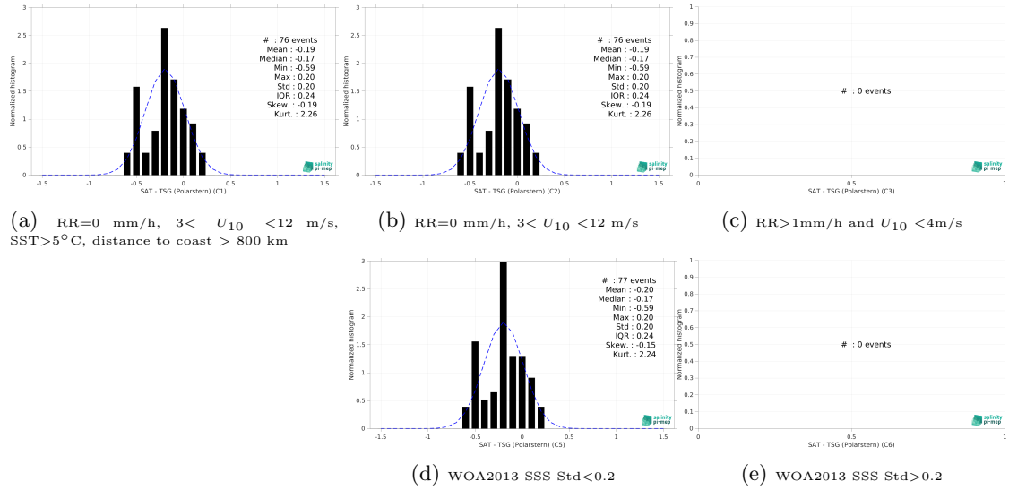
Figure 13: Normalized histogram of \Delta\text{SSS} (Aquarius SSS L2 CAP v5 (JPL) - TSG (Polarstern)) for 5 different subdatasets corresponding to: RR=0 mm/h, 3 < U_{10} < 12 m/s, SST >5^{\circ}\text{C} , distance to coast > 800 km (a), RR=0 mm/h, 3 < U_{10} < 12 m/s (b), RR >1 mm/h and U_{10} < 4 m/s (c), WOA2013 SSS Std <0.2 (d), WOA2013 SSS Std >0.2 (e).
