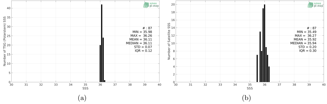
Figure 2: Histograms of SSS from TSG (Polarstern) (a) and Aquarius SSS L2 CAP v5 (JPL) (b) considering all match-up pairs per bins of 0.1 over the Amazon and Orinoco river plumes Pi-MEP region and for the full satellite product period.
