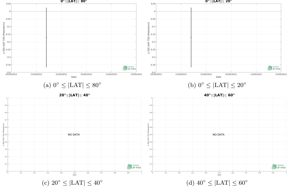
Figure 10: Monthly median (red curves) of \Delta SSS (Satellite - TSG (Polarstern)) and \pm 1 Std (black vertical thick bars) as function of time for all the collected Pi-MEP match-up pairs estimated over the Amazon and Orinoco river plumes Pi-MEP region and for the full satellite product period are shown for different latitude bands: (a) 80°S-80°N, (b) 20°S-20°N, (c) 40°S-20°S and 20°N-40°N and (d) 60°S-40°S and 40°N-60°N.
