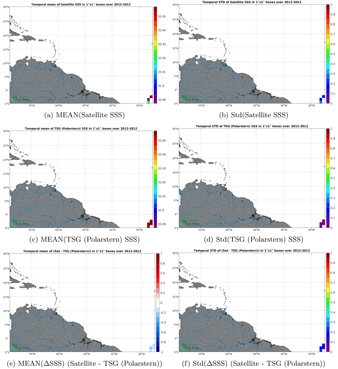
Figure 6: Temporal mean (left) and Std (right) of SSS from Aquarius SSS L2 CAP v5 (JPL) (top), TSG (Polarstern) (middle), and of \Delta SSS (Satellite - TSG (Polarstern)). Only match-up pairs are used to generate these maps.
