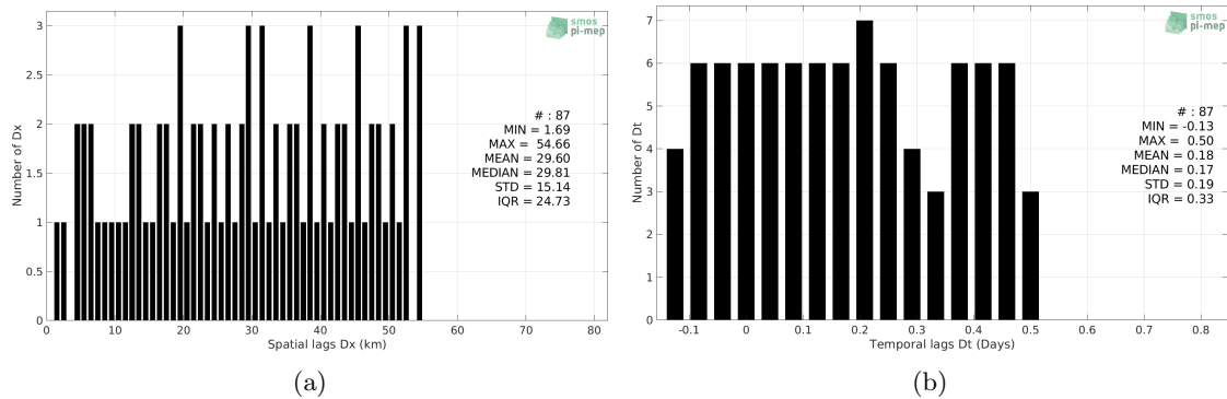
Figure 5: Histograms of the spatial (a) and temporal (b) lags between the location/time of the TSG (Polarstern) measurement and the date of the corresponding Aquarius SSS L2 CAP v5 (JPL) SSS pixel.
