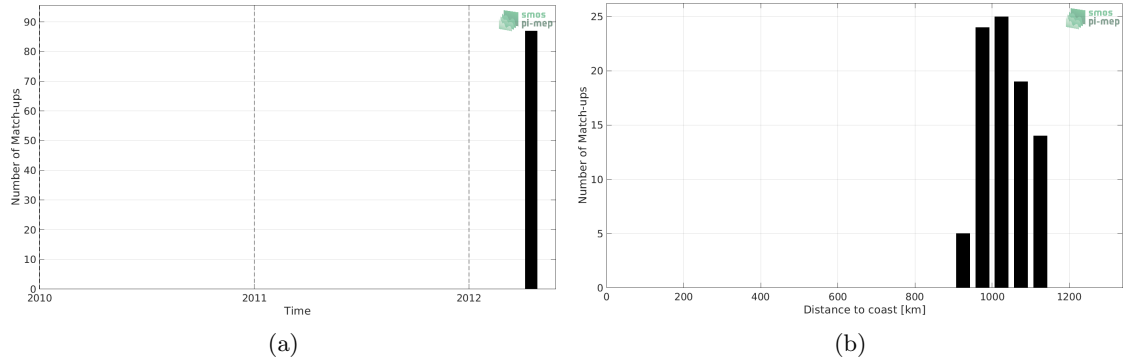
Figure 1: Number of match-ups between TSG (Polarstern) and Aquarius SSS L2 CAP v5 (JPL) SSS as a function of time (a) and as function of the distance to coast (b) over the Amazon and Orinoco river plumes Pi-MEP region and for the full satellite product period.
