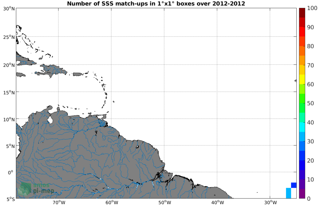
Figure 4: Number of SSS match-ups between TSG (Polarstern) SSS and the Aquarius SSS L2 CAP v5 (JPL) SSS product for the Amazon and Orinoco river plumes Pi-MEP region over 1^\circ \times 1^\circ boxes and for the full satellite product period.
