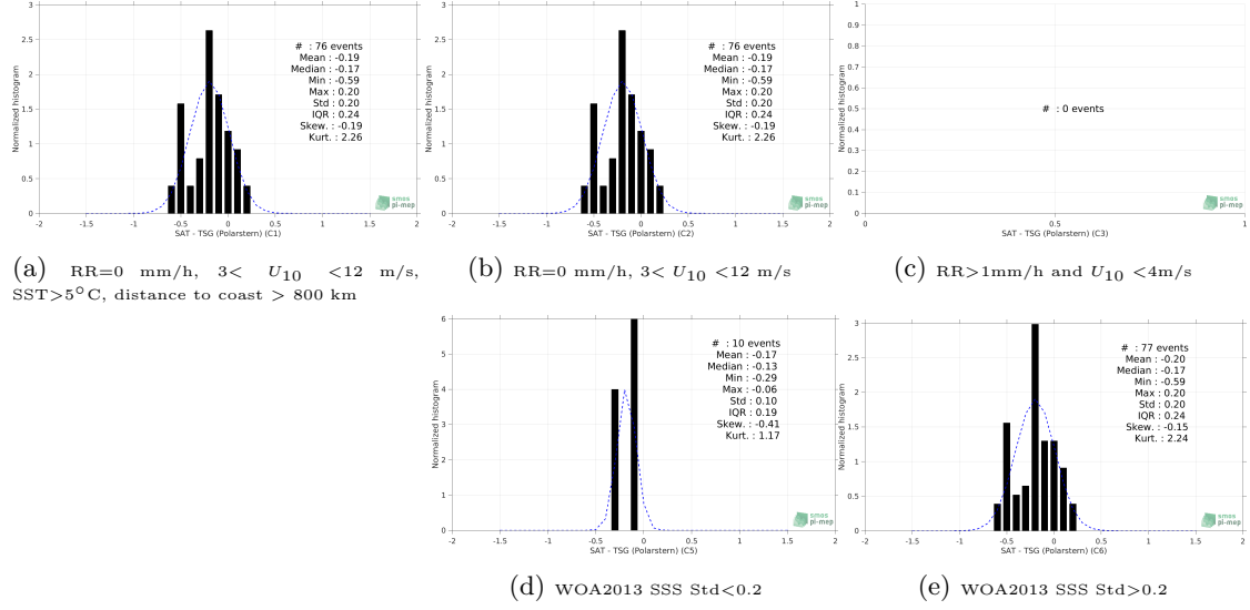
Figure 13: Normalized histogram of \Delta\text{SSS} (Aquarius SSS L2 CAP v5 (JPL) - TSG (Polarstern)) for 5 different subdatasets corresponding to: RR=0 mm/h, 3 < U_{10} < 12 m/s, SST > 5^\circ\text{C} , distance to coast > 800 km (a), RR=0 mm/h, 3 < U_{10} < 12 m/s (b), RR > 1\text{mm/h} and U_{10} < 4\text{m/s} (c), WOA2013 SSS Std < 0.2 (d), WOA2013 SSS Std > 0.2 (e).
