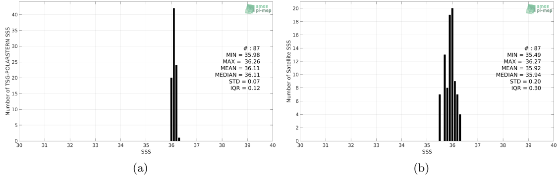
Figure 2: Histograms of SSS from TSG-POLARSTERN (a) and Aquarius-L2-JPL-V5 (b) considering all match-up pairs per bins of 0.1 over the Amazon and Orinoco river plumes Pi-MEP region and for the full satellite product period.
