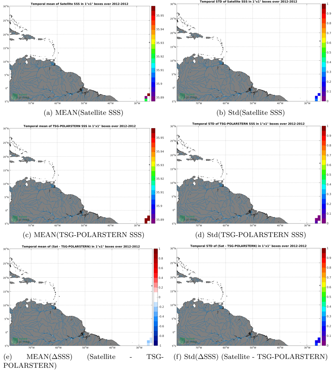
Figure 6: Temporal mean (left) and Std (right) of SSS from Aquarius-L2-JPL-V5 (top), TSG-POLARSTERN (middle), and of \Delta SSS (Satellite - TSG-POLARSTERN). Only match-up pairs are used to generate these maps.
