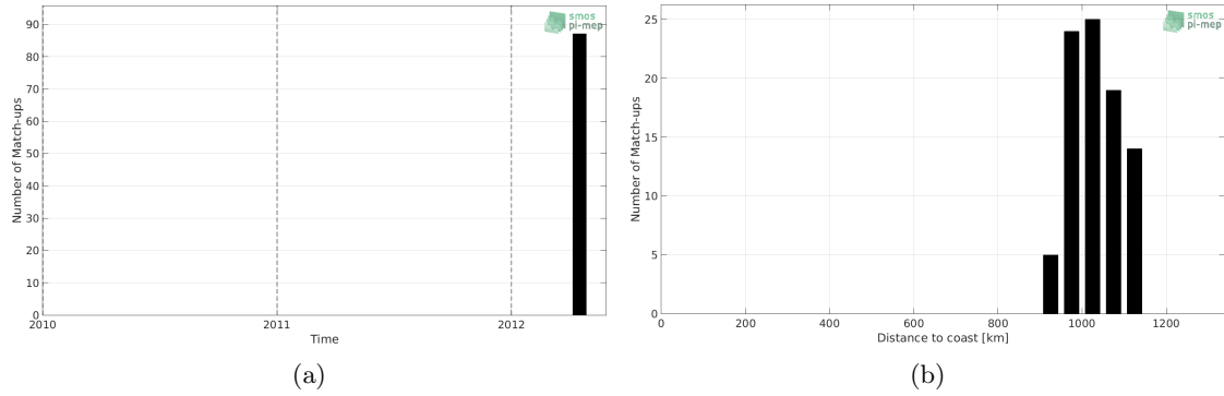
Figure 1: Number of match-ups between TSG-POLARSTERN and Aquarius-L2-JPL-V5 SSS as a function of time (a) and as function of the distance to coast (b) over the Amazon and Orinoco river plumes Pi-MEP region and for the full satellite product period.
