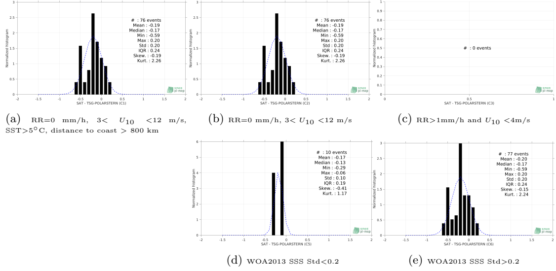
Figure 13: Normalized histogram of \Delta SSS (Aquarius-L2-JPL-V5 - TSG-POLARSTERN) for 5 different subdatasets corresponding to: RR=0 mm/h, 3 < U_{10} < 12 m/s, SST>5°C, distance to coast > 800 km (a), RR=0 mm/h, 3 < U_{10} < 12 m/s (b), RR>1 mm/h and U_{10} < 4 m/s (c), WOA2013 SSS Std<0.2 (d), WOA2013 SSS Std>0.2 (e).
