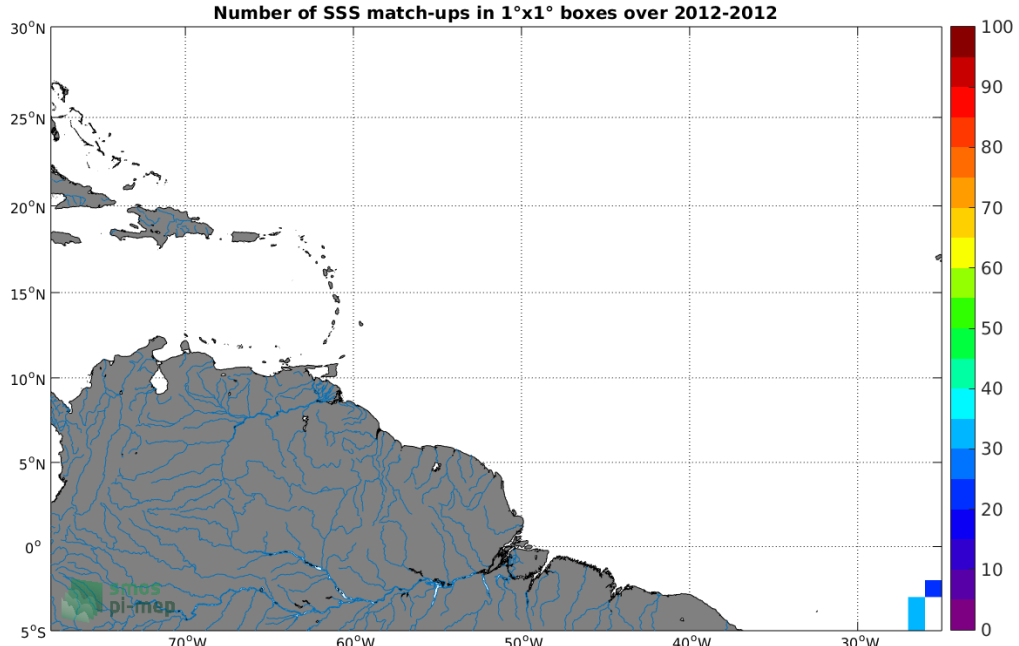
Figure 4: Number of SSS match-ups between TSG-POLARSTERN SSS and the Aquarius-L2-JPL-V5 SSS product for the Amazon and Orinoco river plumes Pi-MEP region over 1^\circ \times 1^\circ boxes and for the full satellite product period.
