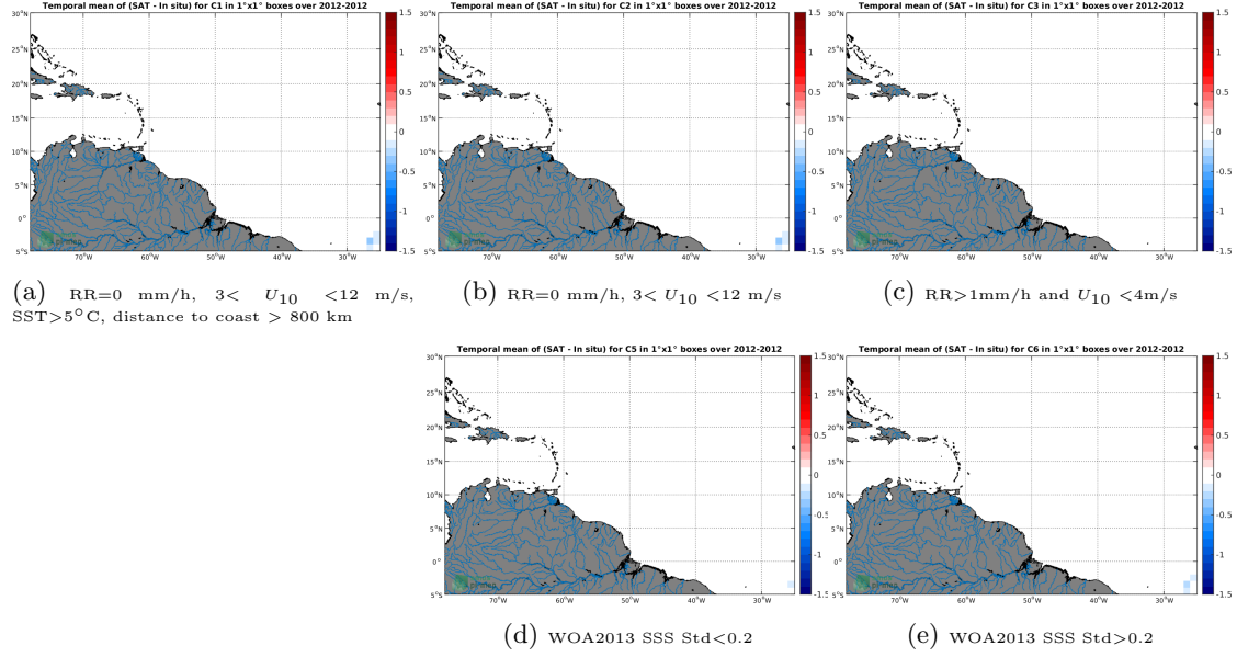
Figure 12: Temporal mean gridded over spatial boxes of size 1^\circ \times 1^\circ of \Delta SSS (Aquarius-L2-JPL-V5 - TSG-POLARSTERN) for 5 different subdatasets corresponding to: RR=0 mm/h, 3 < U_{10} < 12 m/s, SST > 5^\circ C , distance to coast > 800 km (a), RR=0 mm/h, 3 < U_{10} < 12 m/s (b), RR > 1 mm/h and U_{10} < 4 m/s (c), WOA2013 SSS Std < 0.2 (d), WOA2013 SSS Std > 0.2 (e).
