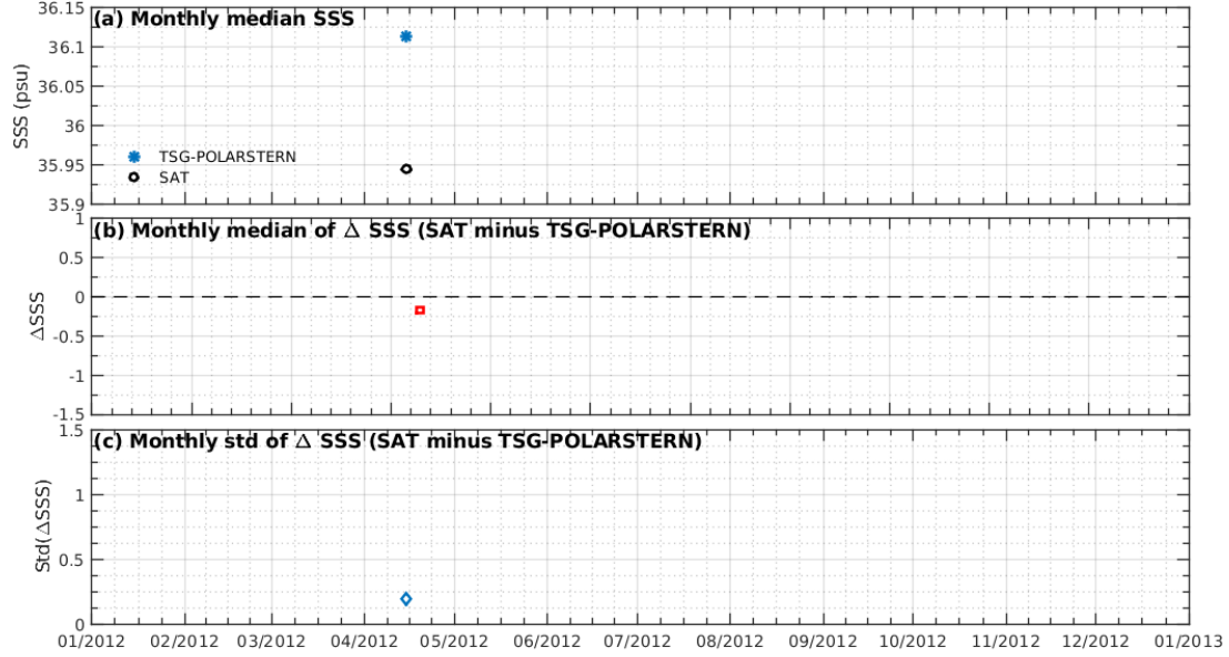
Figure 7: Time series of the monthly median SSS (top), median of \Delta SSS (Satellite - TSG-POLARSTERN) and Std of \Delta SSS (Satellite - TSG-POLARSTERN) over the Amazon and Orinoco river plumes Pi-MEP region considering all match-ups collected by the Pi-MEP.
