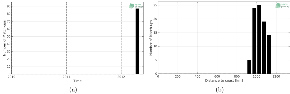
Figure 1: Number of match-ups between TSG-POLARSTERN and Aquarius-L2-JPL-V5 SSS as a function of time (a) and as function of the distance to coast (b) over the Amazon and Orinoco river plumes Pi-MEP region and for the full satellite product period.
