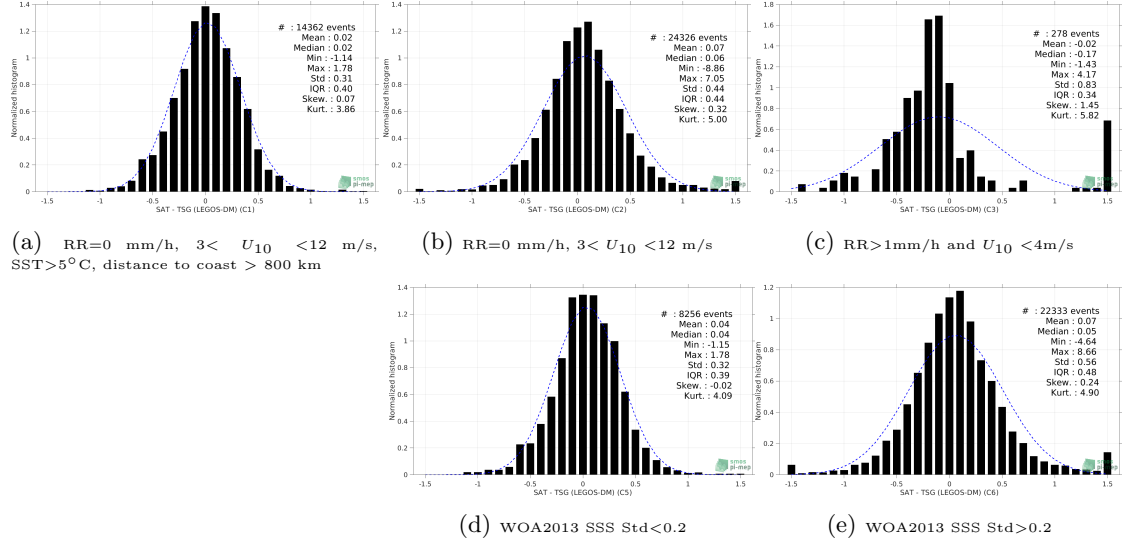
Figure 13: Normalized histogram of \Delta\text{SSS} (Aquarius SSS L2 CAP v5 (JPL) - TSG (LEGOS-DM)) for 5 different subdatasets corresponding to: RR=0 mm/h, 3 < U_{10} < 12 m/s, SST>5°C, distance to coast > 800 km (a), RR=0 mm/h, 3 < U_{10} < 12 m/s (b), RR>1mm/h and U_{10} < 4 m/s (c), WOA2013 SSS Std<0.2 (d), WOA2013 SSS Std>0.2 (e).
