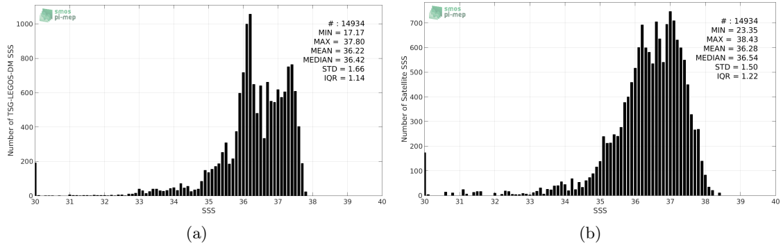
Figure 2: Histograms of SSS from TSG-LEGOS-DM (a) and Aquarius-L2-JPL-V5 (b) considering all match-up pairs per bins of 0.1 over the Amazon and Orinoco river plumes Pi-MEP region and for the full satellite product period.
