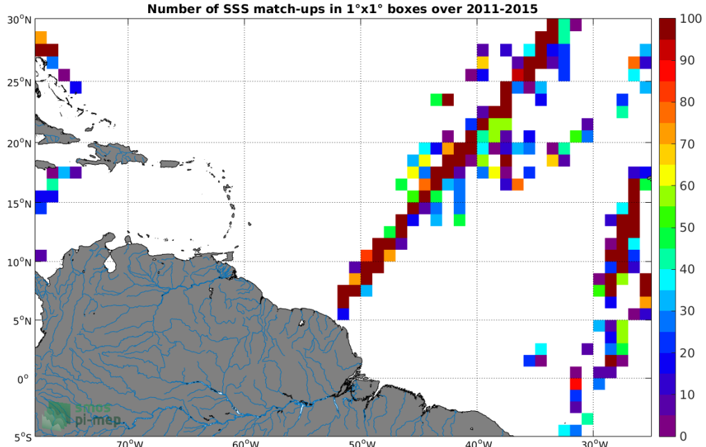
Figure 4: Number of SSS match-ups between TSG-LEGOS-DM SSS and the Aquarius-L2-JPL-V5 SSS product for the Amazon and Orinoco river plumes Pi-MEP region over 1^\circ \times 1^\circ boxes and for the full satellite product period.
