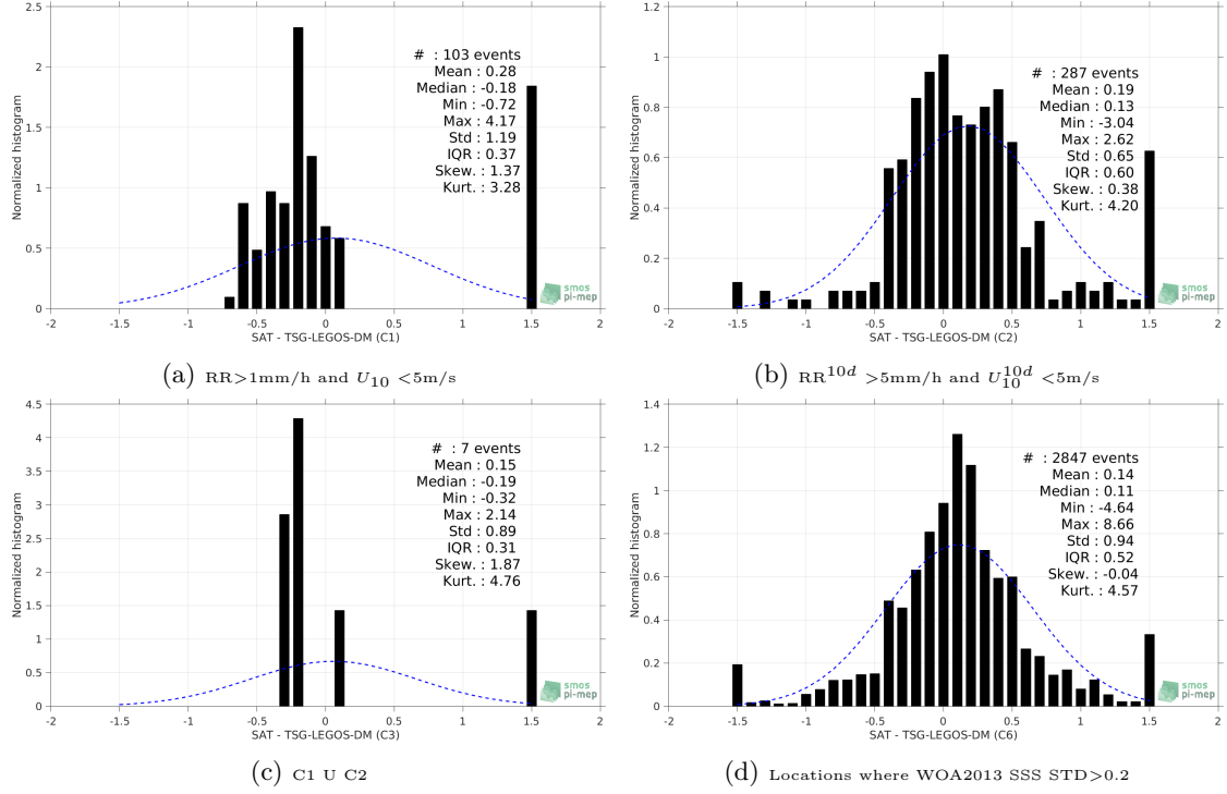
Figure 13: Normalized histogram of \Delta SSS (Aquarius-L2-JPL-V5 - TSG-LEGOS-DM) for 6 different subdatasets corresponding to: RR > 1\text{mm/h} and U_{10} < 5\text{m/s} (a), RR^{10d} > 5\text{mm/h} and U_{10}^{10d} < 5\text{m/s} (b), C1 U C2 (c), Locations where WOA2013 SSS STD > 0.2 (d).
