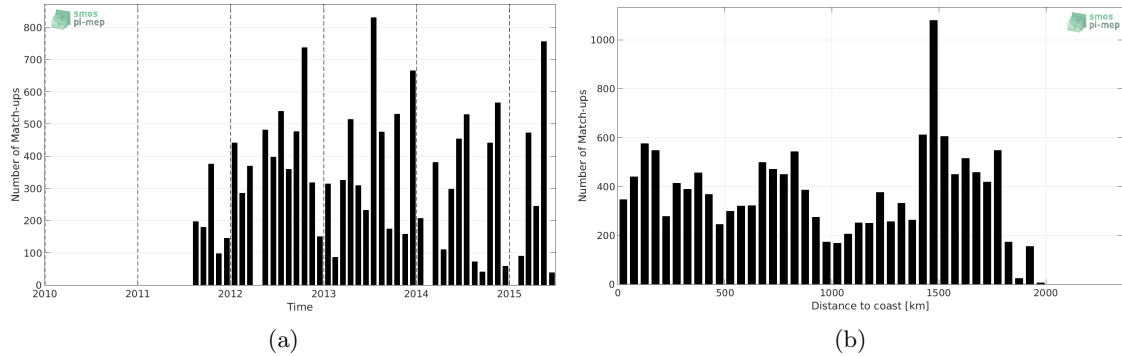
Figure 1: Number of match-ups between TSG-LEGOS-DM and Aquarius-L2-JPL-V5 SSS as a function of time (a) and as function of the distance to coast (b) over the Amazon and Orinoco river plumes Pi-MEP region and for the full satellite product period.
