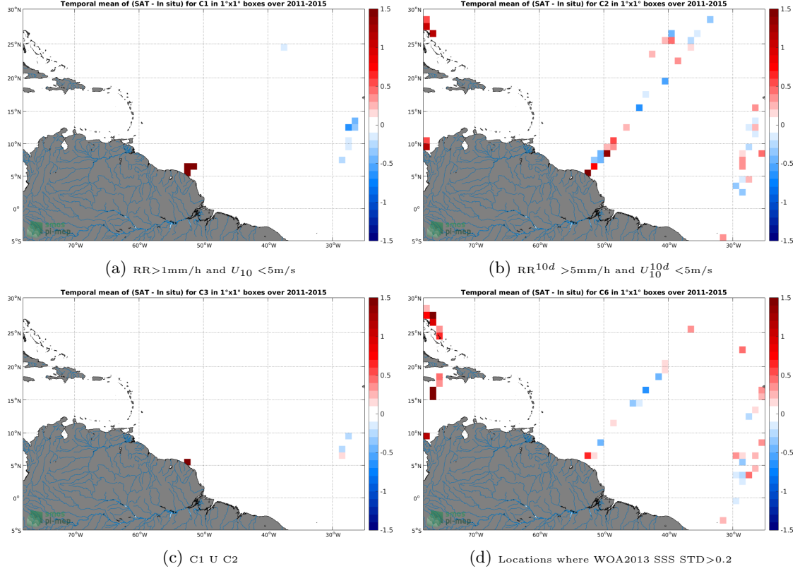
Figure 12: Temporal mean gridded over spatial boxes of size 1^\circ \times 1^\circ of \Delta SSS (Aquarius-L2-JPL-V5 - TSG-LEGOS-DM) for 4 different subdatasets corresponding to: RR > 1\text{mm/h} and U_{10} < 5\text{m/s} (a), RR^{10d} > 5\text{mm/h} and U_{10}^{10d} < 5\text{m/s} (b), C1 U C2 (c), Locations where WOA2013 SSS STD > 0.2 (d).
