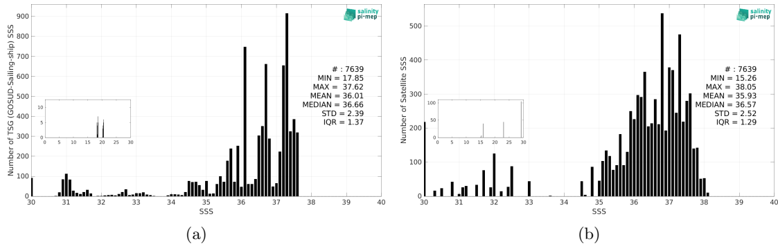
Figure 3: Histograms of SSS from TSG (GOSUD-Sailing-ship) (a) and Aquarius SSS L2 CAP v5 (JPL) (b) considering all match-up pairs per bins of 0.1 over the Amazon and Orinoco river plumes Pi-MEP region and for the full satellite product period.
