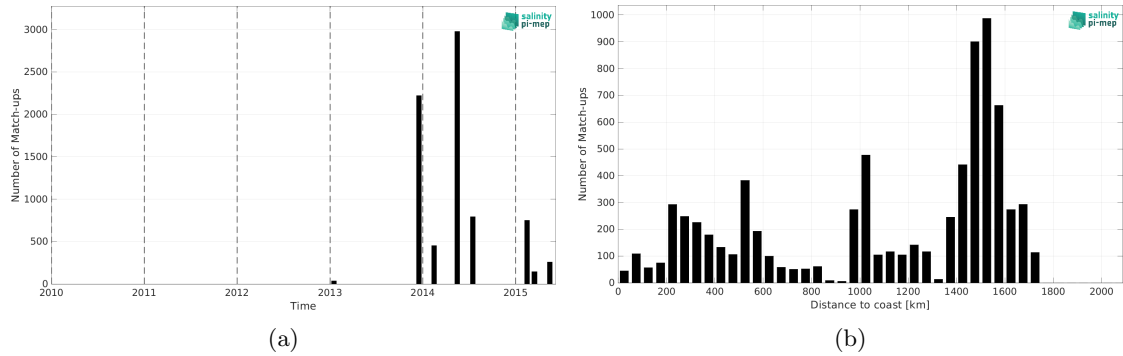
Figure 2: Number of match-ups between TSG (GOSUD-Sailing-ship) and Aquarius SSS L2 CAP v5 (JPL) SSS as a function of time (a) and as function of the distance to coast (b) over the Amazon and Orinoco river plumes Pi-MEP region and for the full satellite product period.
