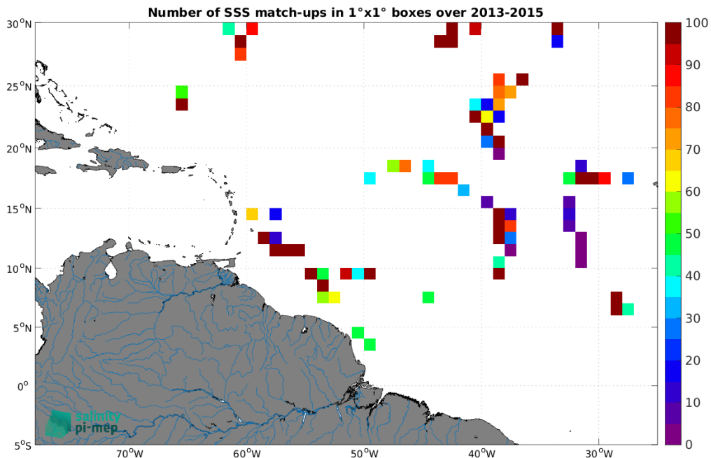
Figure 5: Number of SSS match-ups between TSG (GOSUD-Sailing-ship) SSS and the Aquarius SSS L2 CAP v5 (JPL) SSS product for the Amazon and Orinoco river plumes Pi-MEP region over 1^\circ \times 1^\circ boxes and for the full satellite product period.
