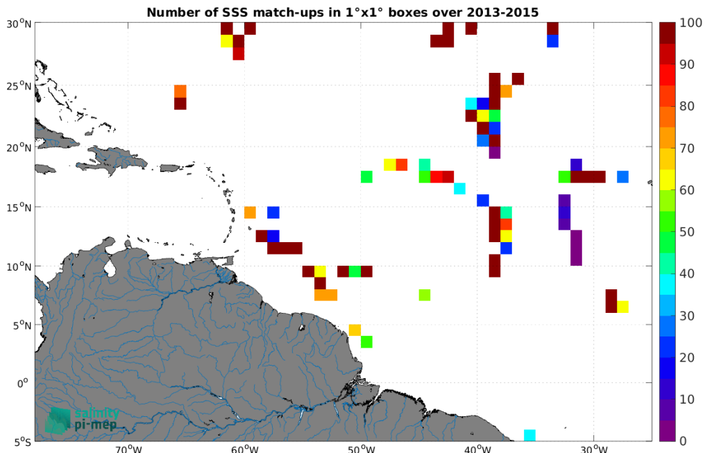
Figure 4: Number of SSS match-ups between TSG (GOSUD-Sailing-ship) SSS and the Aquarius SSS L2 CAP v5 (JPL) SSS product for the Amazon and Orinoco river plumes Pi-MEP region over 1^\circ \times 1^\circ boxes and for the full satellite product period.
