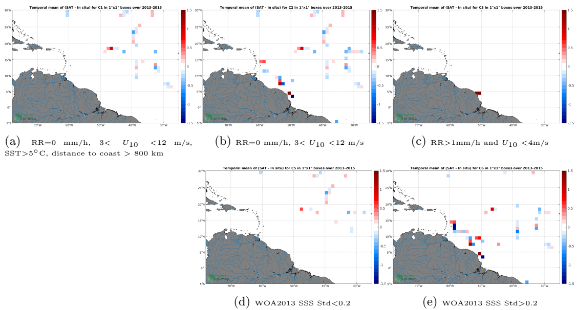
Figure 12: Temporal mean gridded over spatial boxes of size 1°x1° of \Delta SSS (Aquarius SSS L2 CAP v5 (JPL) - TSG (GOSUD-Sailing-ship)) for 5 different subdatasets corresponding to: RR=0 mm/h, 3 < U_{10} < 12 m/s, SST > 5°C, distance to coast > 800 km (a), RR=0 mm/h, 3 < U_{10} < 12 m/s (b), RR > 1mm/h and U_{10} < 4 m/s (c), WOA2013 SSS Std < 0.2 (d), WOA2013 SSS Std > 0.2 (e).
