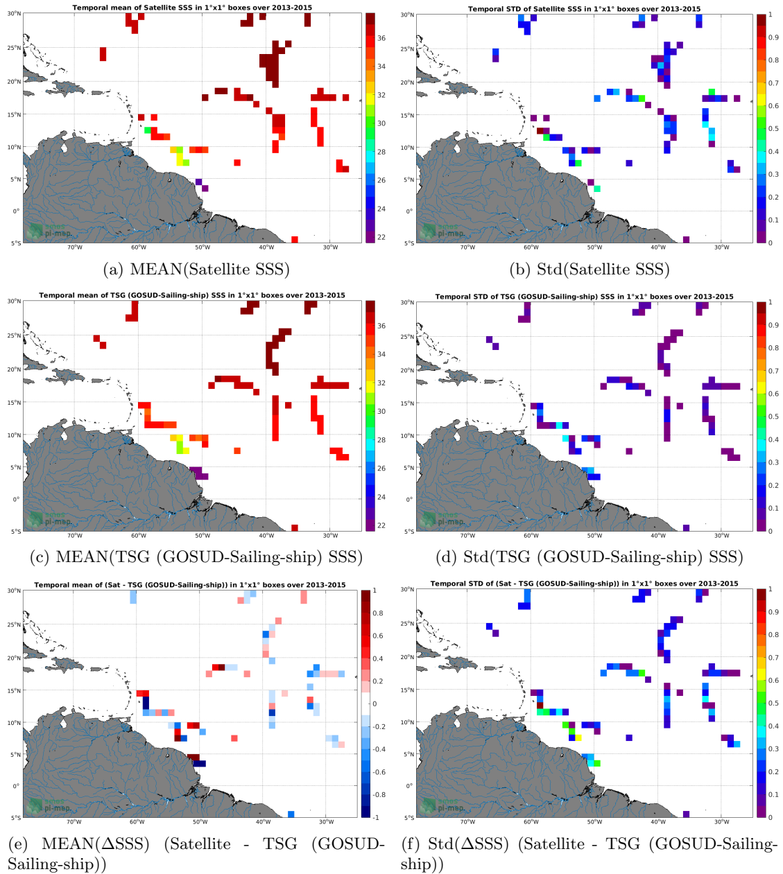
Figure 6: Temporal mean (left) and Std (right) of SSS from Aquarius SSS L2 CAP v5 (JPL) (top), TSG (GOSUD-Sailing-ship) (middle), and of \Delta SSS (Satellite - TSG (GOSUD-Sailing-ship)). Only match-up pairs are used to generate these maps.
