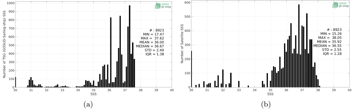
Figure 2: Histograms of SSS from TSG (GOSUD-Sailing-ship) (a) and Aquarius SSS L2 CAP v5 (JPL) (b) considering all match-up pairs per bins of 0.1 over the Amazon and Orinoco river plumes Pi-MEP region and for the full satellite product period.
