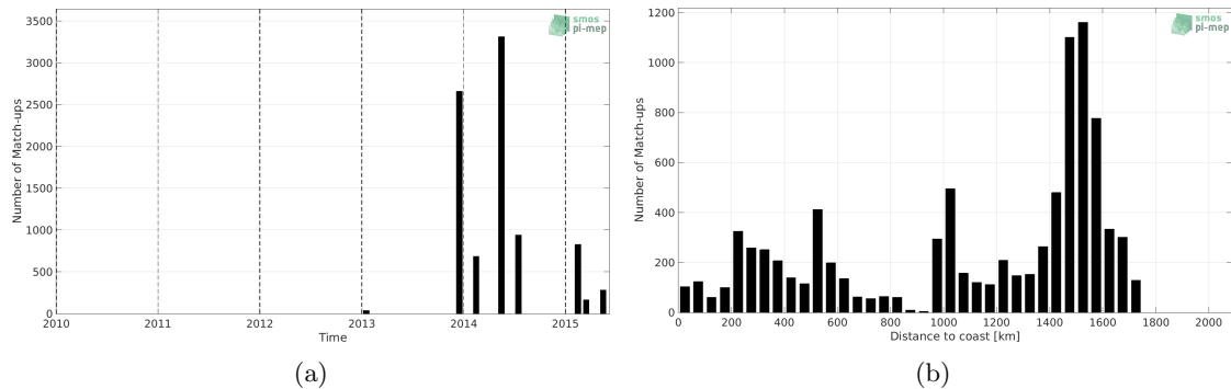
Figure 1: Number of match-ups between TSG (GOSUD-Sailing-ship) and Aquarius SSS L2 CAP v5 (JPL) SSS as a function of time (a) and as function of the distance to coast (b) over the Amazon and Orinoco river plumes Pi-MEP region and for the full satellite product period.
