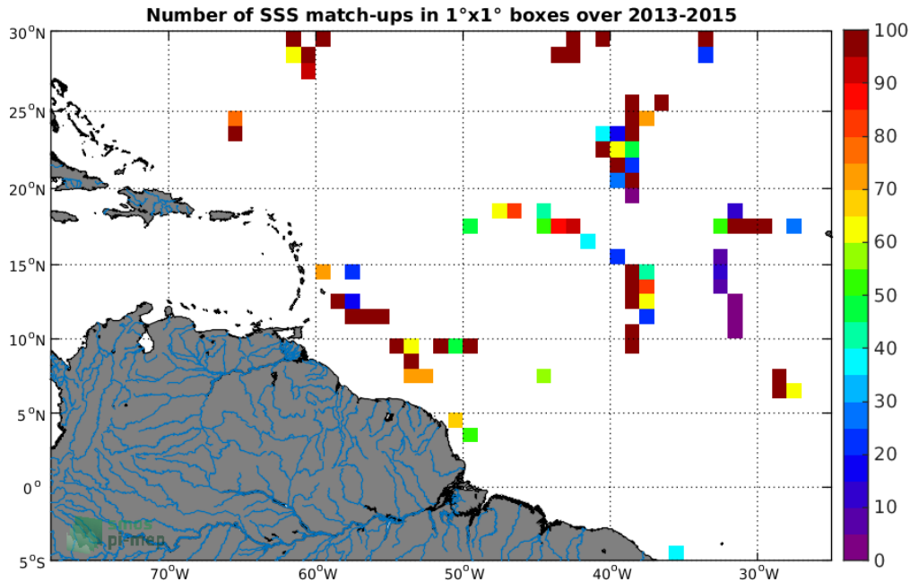
Figure 4: Number of SSS match-ups between TSG-GOSUD-Sailing-ship SSS and the Aquarius-L2-JPL-V5 SSS product for the Amazon and Orinoco river plumes Pi-MEP region over 1^\circ \times 1^\circ boxes and for the full satellite product period.
