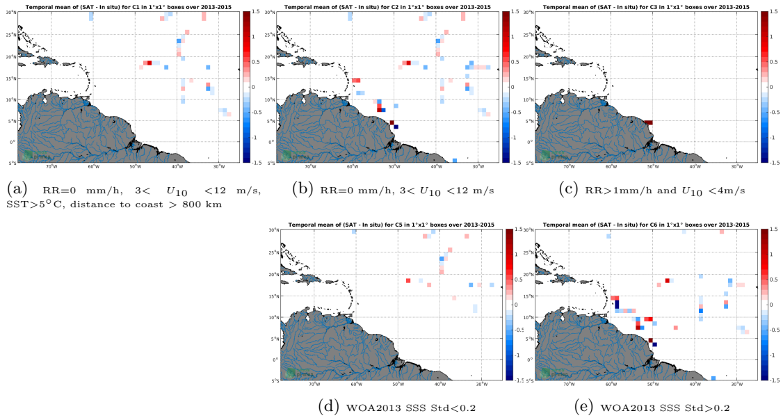
Figure 12: Temporal mean gridded over spatial boxes of size 1^\circ \times 1^\circ of \Delta SSS (Aquarius-L2-JPL-V5 - TSG-GOSUD-Sailing-ship) for 5 different subdatasets corresponding to:RR=0 mm/h, 3 < U_{10} < 12 m/s, SST>5°C, distance to coast > 800 km (a), RR=0 mm/h, 3 < U_{10} < 12 m/s (b), RR>1mm/h and U_{10} < 4 m/s (c), WOA2013 SSS Std<0.2 (d), WOA2013 SSS Std>0.2 (e).
