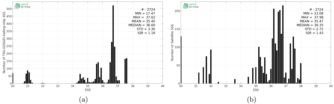
Figure 2: Histograms of SSS from TSG-GOSUD-Sailing-ship (a) and Aquarius-L2-JPL-V5 (b) considering all match-up pairs per bins of 0.1 over the Amazon and Orinoco river plumes Pi-MEP region and for the full satellite product period.
