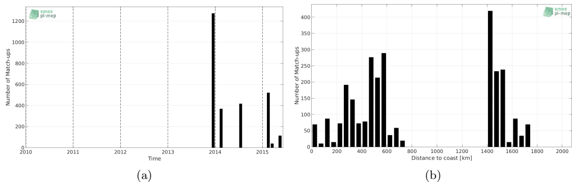
Figure 1: Number of match-ups between TSG-GOSUD-Sailing-ship and Aquarius-L2-JPL-V5 SSS as a function of time (a) and as function of the distance to coast (b) over the Amazon and Orinoco river plumes Pi-MEP region and for the full satellite product period.
