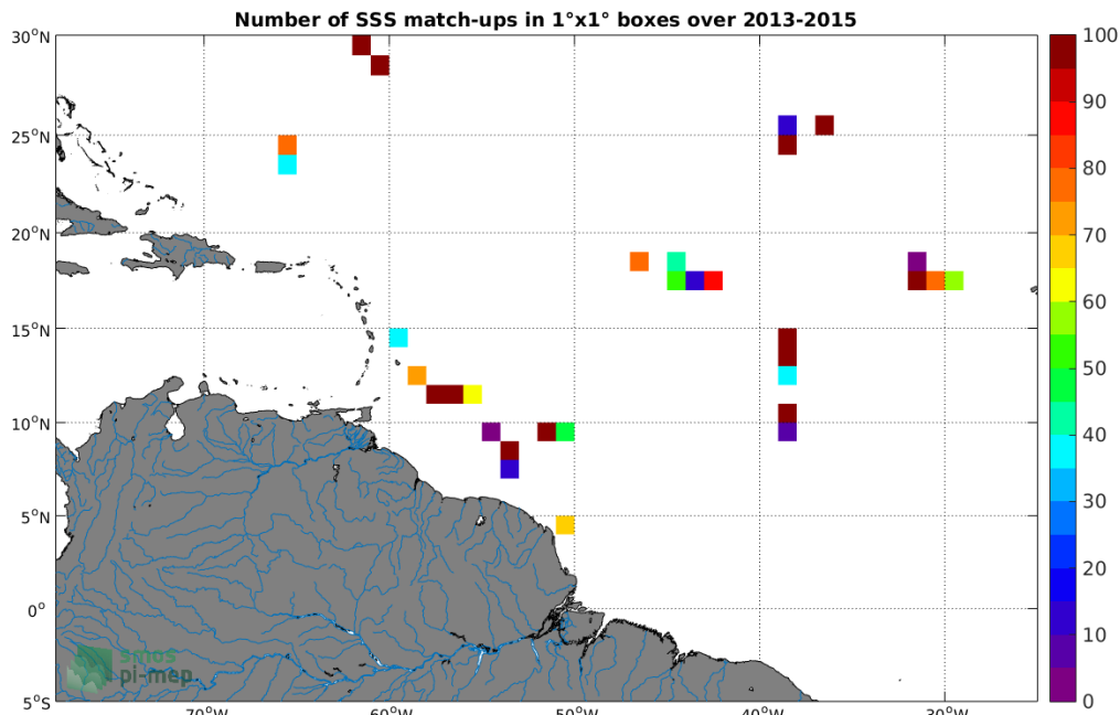
Figure 4: Number of SSS match-ups between TSG-GOSUD-Sailing-ship SSS and the Aquarius-L2-JPL-V5 SSS product for the Amazon and Orinoco river plumes Pi-MEP region over 1°x1° boxes and for the full satellite product period.
