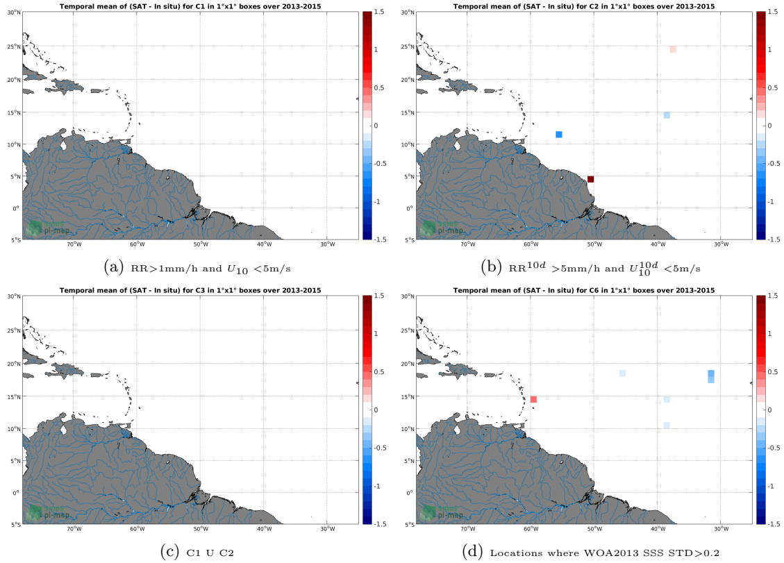
Figure 12: Temporal mean gridded over spatial boxes of size 1^\circ \times 1^\circ of \Delta SSS (Aquarius-L2-JPL-V5 - TSG-GOSUD-Sailing-ship) for 4 different subdatasets corresponding to: RR > 1mm/h and U_{10} < 5\text{m/s} (a), RR^{10d} > 5\text{mm/h} and U_{10}^{10d} < 5\text{m/s} (b), C1 U C2 (c), Locations where WOA2013 SSS STD > 0.2 (d).
