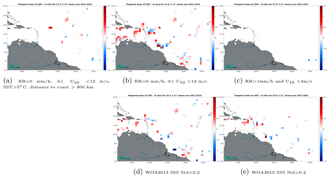
Figure 14: Temporal mean gridded over spatial boxes of size 1^\circ \times 1^\circ of \Delta\text{SSS} (Aquarius SSS L2 CAP v5 (JPL) - TSG (GOSUD-Research-vessel)) for 5 different subdatasets corresponding to:RR=0 mm/h, 3 < U_{10} < 12 m/s, SST >5^\circ\text{C} , distance to coast > 800 km (a), RR=0 mm/h, 3 < U_{10} < 12 m/s (b), RR >1 mm/h and U_{10} < 4 m/s (c), WOA2013 SSS Std <0.2 (d), WOA2013 SSS Std >0.2 (e).
