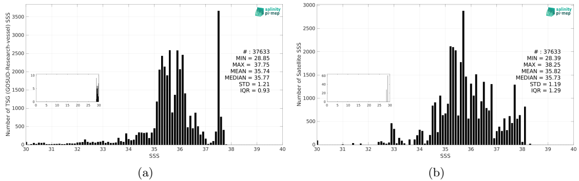
Figure 3: Histograms of SSS from TSG (GOSUD-Research-vessel) (a) and Aquarius SSS L2 CAP v5 (JPL) (b) considering all match-up pairs per bins of 0.1 over the Amazon and Orinoco river plumes Pi-MEP region and for the full satellite product period.
