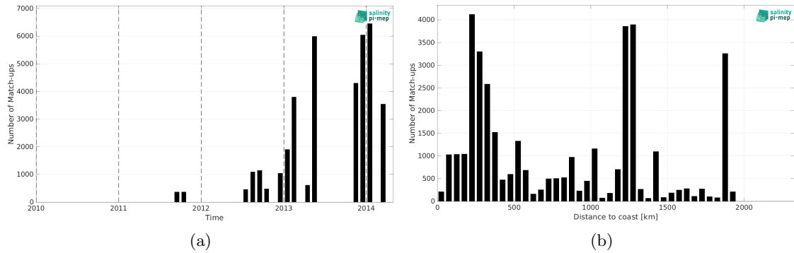
Figure 2: Number of match-ups between TSG (GOSUD-Research-vessel) and Aquarius SSS L2 CAP v5 (JPL) SSS as a function of time (a) and as function of the distance to coast (b) over the Amazon and Orinoco river plumes Pi-MEP region and for the full satellite product period.
