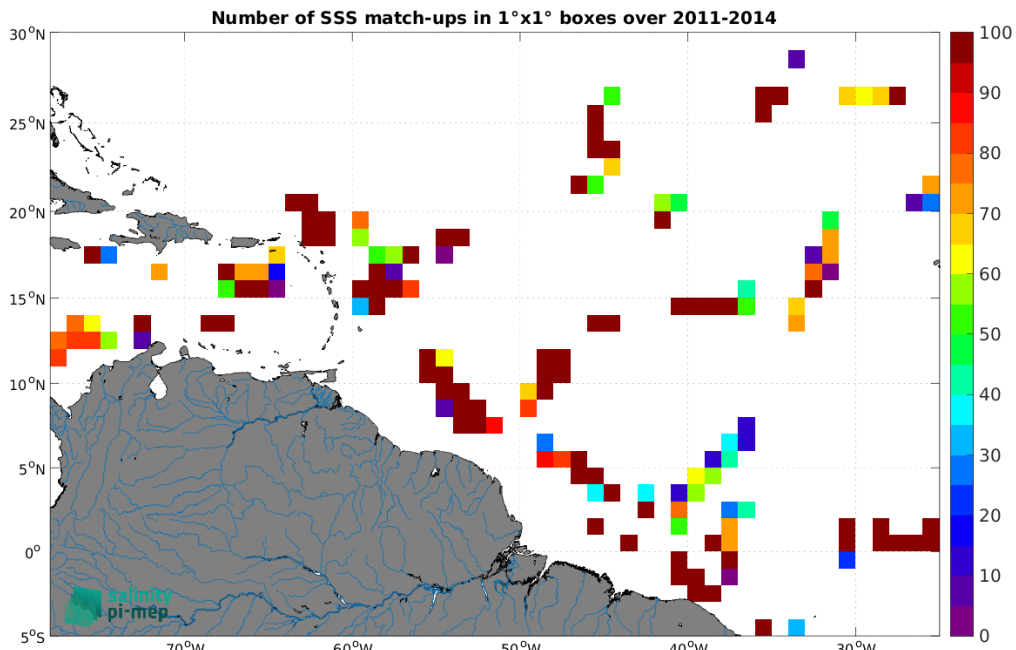
Figure 5: Number of SSS match-ups between TSG (GOSUD-Research-vessel) SSS and the Aquarius SSS L2 CAP v5 (JPL) SSS product for the Amazon and Orinoco river plumes Pi-MEP region over 1^\circ \times 1^\circ boxes and for the full satellite product period.
