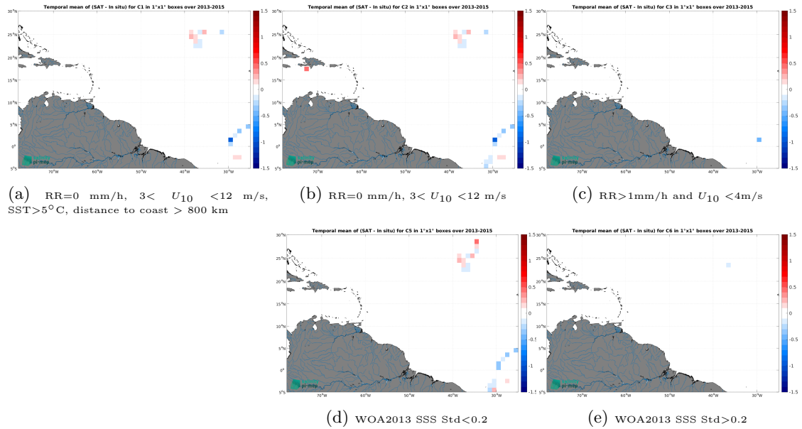
Figure 12: Temporal mean gridded over spatial boxes of size 1^\circ \times 1^\circ of \Delta SSS (Aquarius SSS L2 CAP v5 (JPL) - TSG (CSIC-UTM)) for 5 different subdatasets corresponding to:RR=0 mm/h, 3 < U_{10} < 12 m/s, SST >5^\circ C, distance to coast > 800 km (a), RR=0 mm/h, 3 < U_{10} < 12 m/s (b), RR >1 mm/h and U_{10} < 4 m/s (c), WOA2013 SSS Std <0.2 (d), WOA2013 SSS Std >0.2 (e).
