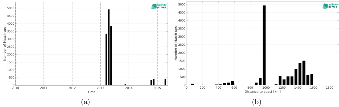
Figure 1: Number of match-ups between TSG (CSIC-UTM) and Aquarius SSS L2 CAP v5 (JPL) SSS as a function of time (a) and as function of the distance to coast (b) over the Amazon and Orinoco river plumes Pi-MEP region and for the full satellite product period.
