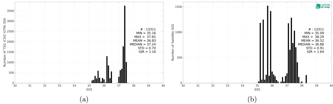
Figure 2: Histograms of SSS from TSG (CSIC-UTM) (a) and Aquarius SSS L2 CAP v5 (JPL) (b) considering all match-up pairs per bins of 0.1 over the Amazon and Orinoco river plumes Pi-MEP region and for the full satellite product period.
