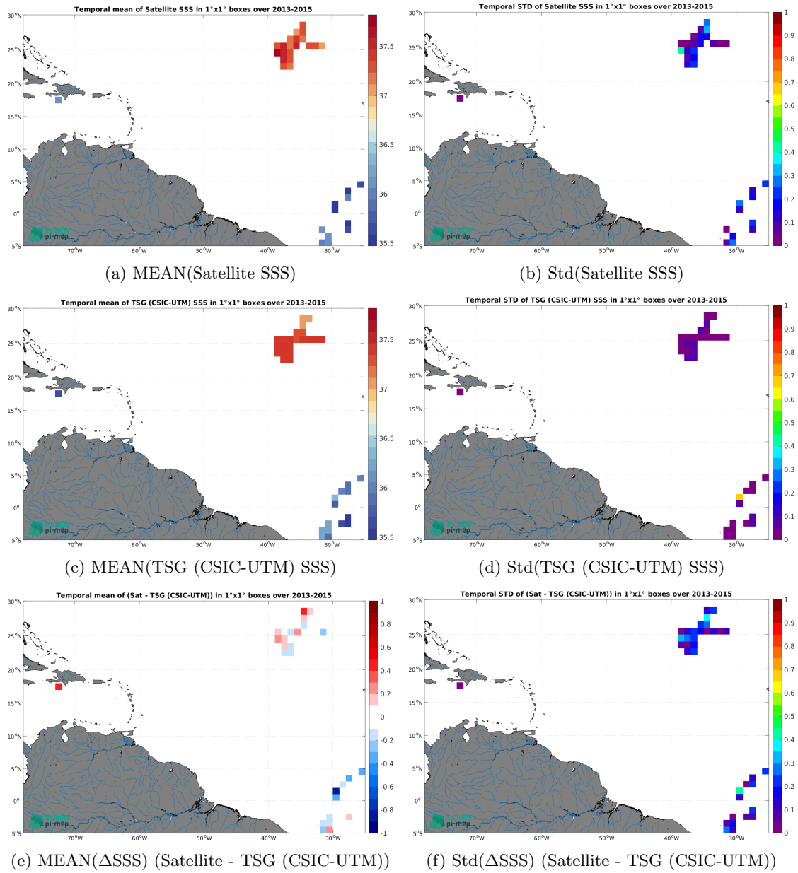
Figure 6: Temporal mean (left) and Std (right) of SSS from Aquarius SSS L2 CAP v5 (JPL) (top), TSG (CSIC-UTM) (middle), and of \Delta SSS (Satellite - TSG (CSIC-UTM)). Only match-up pairs are used to generate these maps.
