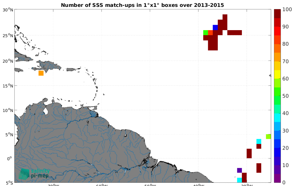
Figure 4: Number of SSS match-ups between TSG (CSIC-UTM) SSS and the Aquarius SSS L2 CAP v5 (JPL) SSS product for the Amazon and Orinoco river plumes Pi-MEP region over 1^\circ \times 1^\circ boxes and for the full satellite product period.
