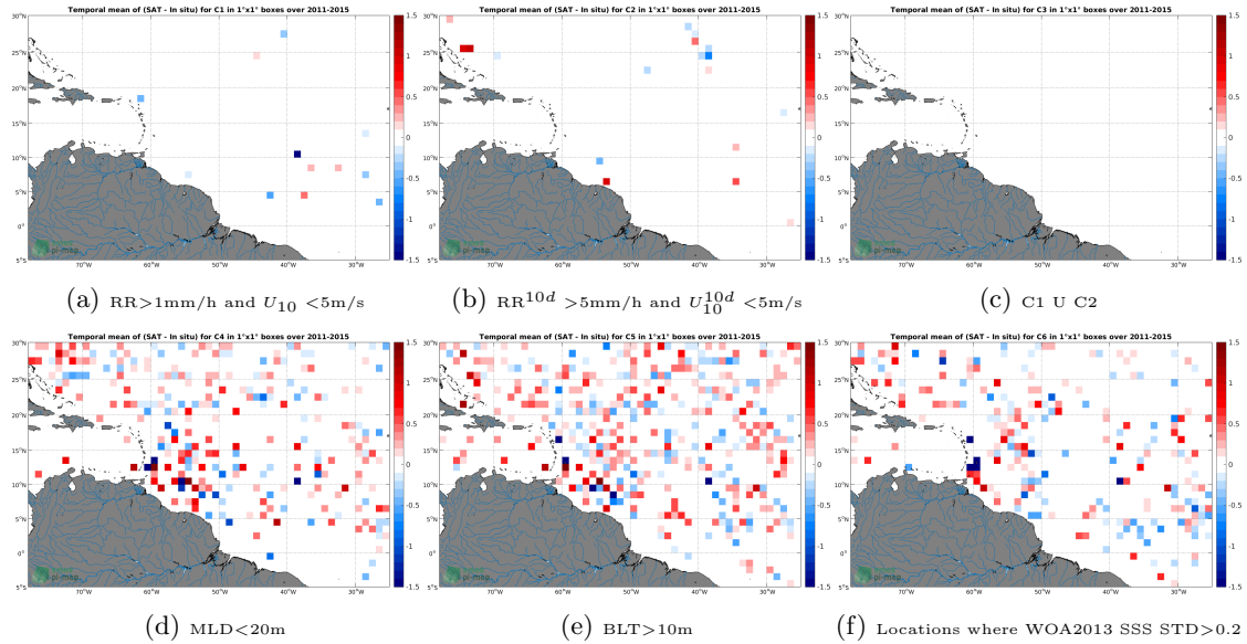
Figure 12: Temporal mean gridded over spatial boxes of size 1^\circ \times 1^\circ of \Delta SSS (Aquarius-L2-JPL-V5 - Argo) for 6 different subdatasets corresponding to: RR > 1\text{mm/h} and U_{10} < 5\text{m/s} (a), RR^{10d} > 5\text{mm/h} and U_{10}^{10d} < 5\text{m/s} (b), C1 U C2 (c), MLD < 20\text{m} (d), BLT > 10\text{m} (e), Locations where WOA2013 SSS STD > 0.2 (f).
