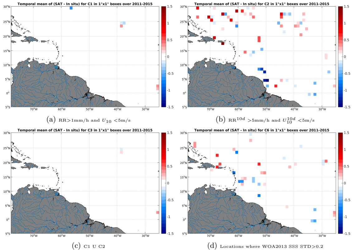
Figure 12: Temporal mean gridded over spatial boxes of size 1^\circ \times 1^\circ of \Delta SSS (AQUARIUS-L2-JPL-V4 - TSG-SAMOS) for 4 different subdatasets corresponding to: RR > 1\text{mm/h} and U_{10} < 5\text{m/s} (a), RR^{10d} > 5\text{mm/h} and U_{10}^{10d} < 5\text{m/s} (b), C1 U C2 (c), Locations where WOA2013 SSS STD > 0.2 (d).
