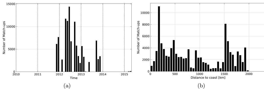
Figure 1: Number of match-ups between TSG-SAMOS and AQUARIUS-L2-JPL-V4 SSS as a function of time (a) and as function of the distance to coast (b) over the Amazon and Orinoco river plumes Pi-MEP region and for the full satellite product period.
