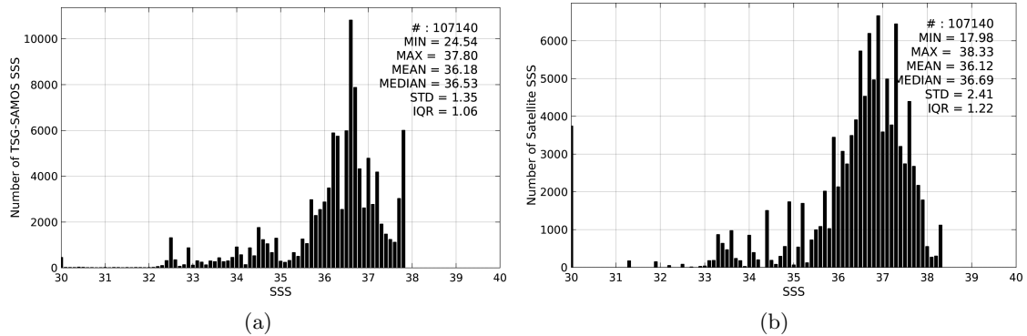
Figure 2: Histograms of SSS from TSG-SAMOS (a) and AQUARIUS-L2-JPL-V4 (b) considering all match-up pairs per bins of 0.1 over the Amazon and Orinoco river plumes Pi-MEP region and for the full satellite product period.
