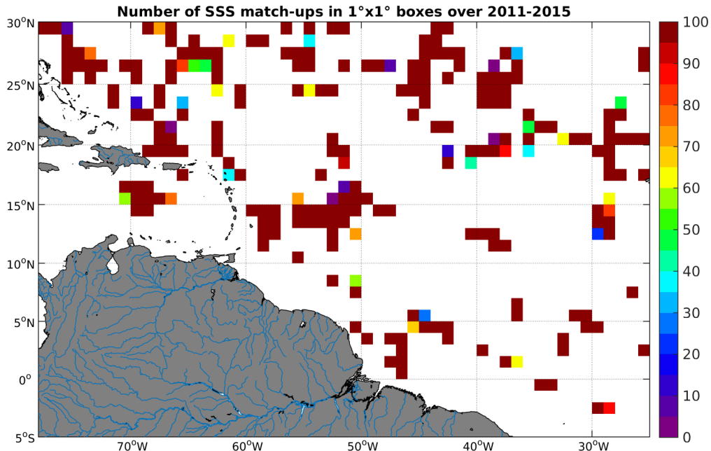
Figure 4: Number of SSS match-ups between TSG-SAMOS SSS and the AQUARIUS-L2-JPL-V4 SSS product for the Amazon and Orinoco river plumes Pi-MEP region over 1^\circ \times 1^\circ boxes and for the full satellite product period.
