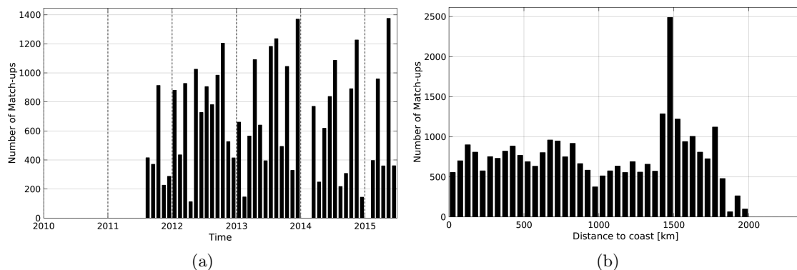
Figure 1: Number of match-ups between TSG-LEGOS-DM and AQUARIUS-L2-JPL-V4 SSS as a function of time (a) and as function of the distance to coast (b) over the Amazon and Orinoco river plumes Pi-MEP region and for the full satellite product period.
