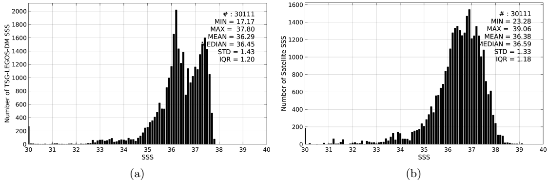
Figure 2: Histograms of SSS from TSG-LEGOS-DM (a) and AQUARIUS-L2-JPL-V4 (b) considering all match-up pairs per bins of 0.1 over the Amazon and Orinoco river plumes Pi-MEP region and for the full satellite product period.
