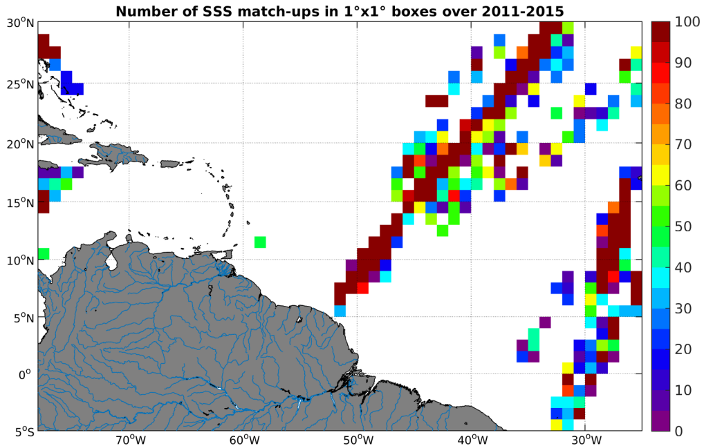
Figure 4: Number of SSS match-ups between TSG-LEGOS-DM SSS and the AQUARIUS-L2-JPL-V4 SSS product for the Amazon and Orinoco river plumes Pi-MEP region over 1^\circ \times 1^\circ boxes and for the full satellite product period.
