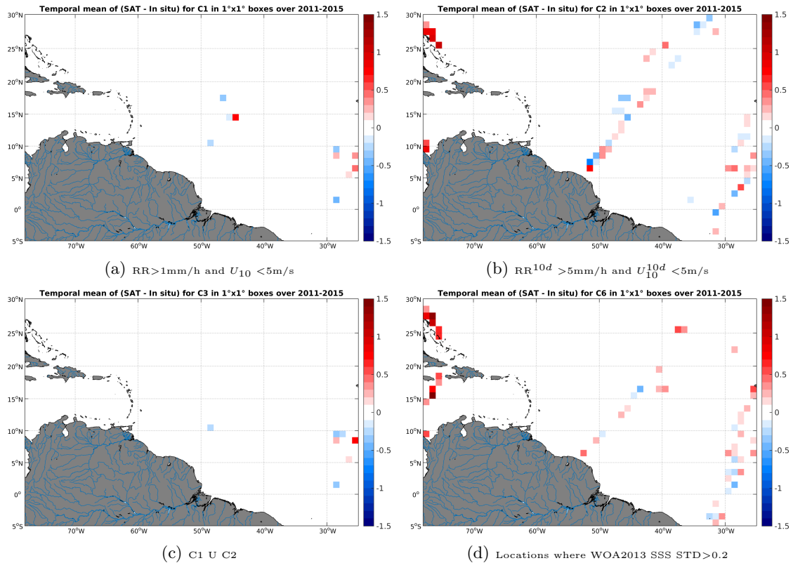
Figure 12: Temporal mean gridded over spatial boxes of size 1^\circ \times 1^\circ of \Delta SSS (AQUARIUS-L2-JPL-V4 - TSG-LEGOS-DM) for 4 different subdatasets corresponding to: RR > 1\text{mm/h} and U_{10} < 5\text{m/s} (a), RR^{10d} > 5\text{mm/h} and U_{10}^{10d} < 5\text{m/s} (b), C1 U C2 (c), Locations where WOA2013 SSS STD > 0.2 (d).
