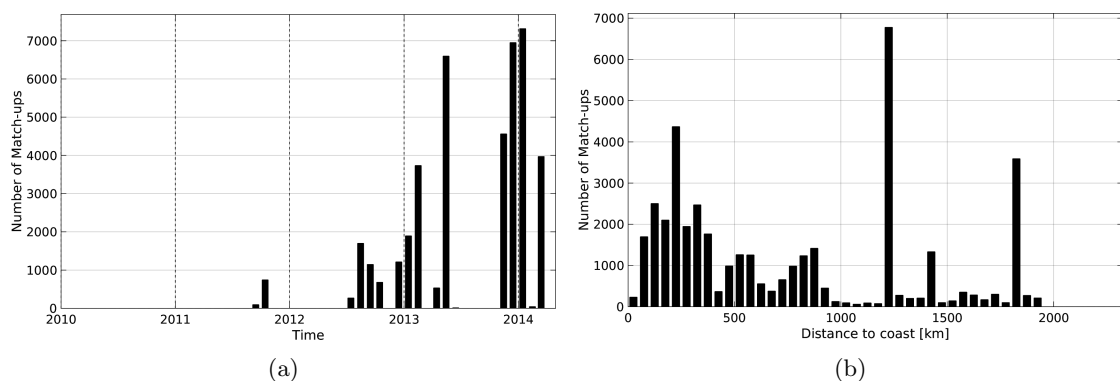
Figure 1: Number of match-ups between TSG-GOSUD-Research-vessel and AQUARIUS-L2-JPL-V4 SSS as a function of time (a) and as function of the distance to coast (b) over the Amazon and Orinoco river plumes Pi-MEP region and for the full satellite product period.
