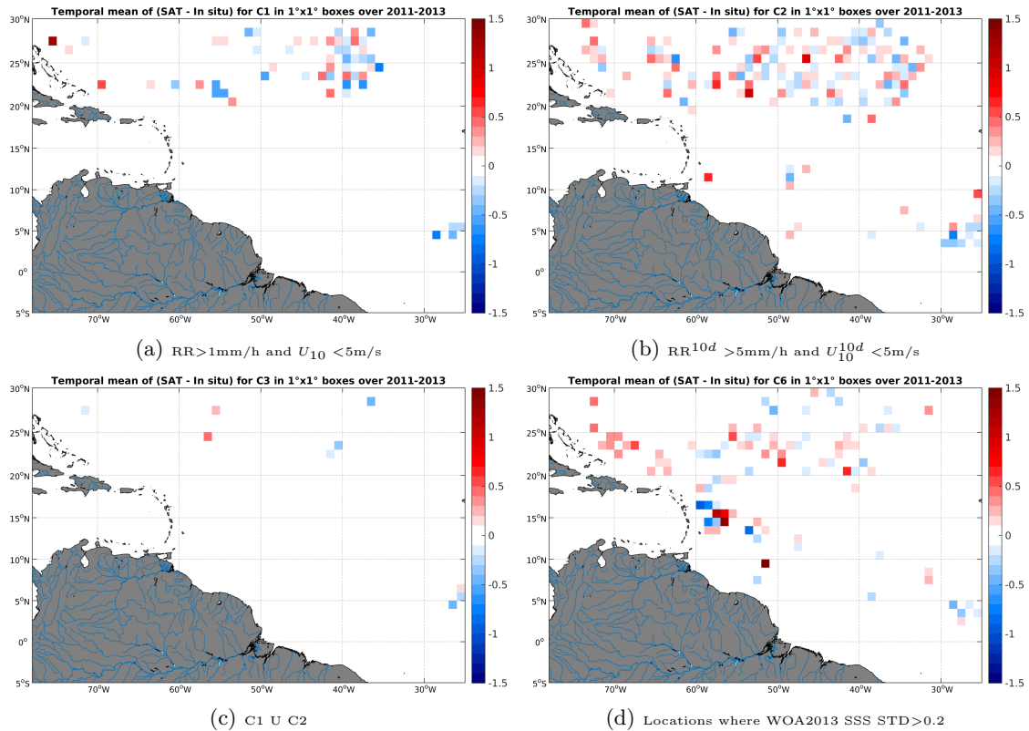
Figure 11: Temporal mean gridded over spatial boxes of size 1^\circ \times 1^\circ of \Delta SSS (AQUARIUS-L2-JPL-V4 - Surface drifters) for 4 different subdatasets corresponding to: RR > 1mm/h and U_{10} < 5 m/s (a), RR^{10d} > 5 mm/h and U_{10}^{10d} < 5 m/s (b), C1 U C2 (c), Locations where WOA2013 SSS STD > 0.2 (d).
