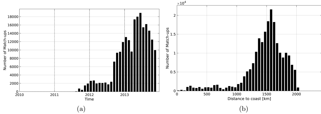
Figure 1: Number of match-ups between Surface drifters and AQUARIUS-L2-JPL-V4 SSS as a function of time (a) and as function of the distance to coast (b) over the Amazon and Orinoco river plumes Pi-MEP region and for the full satellite product period.
