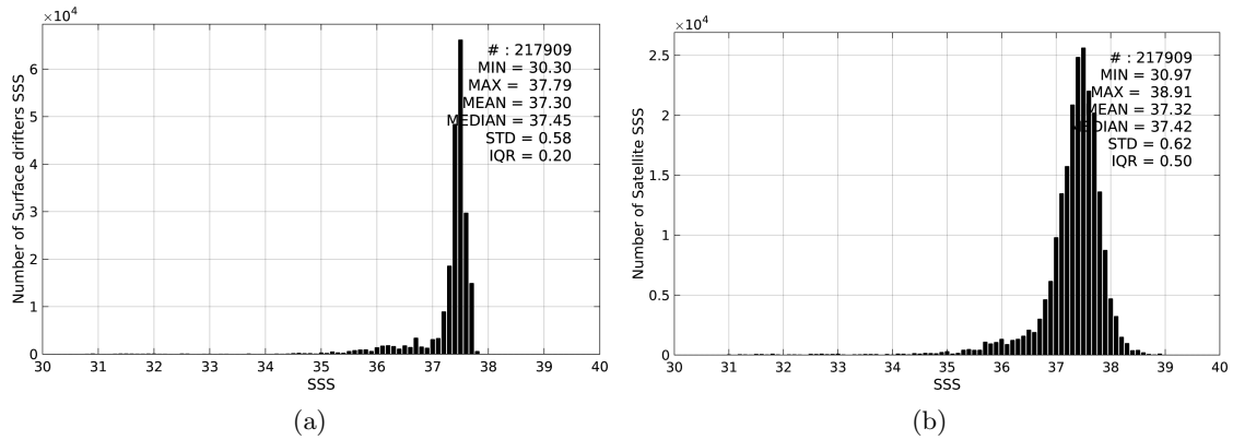
Figure 2: Histograms of SSS from Surface drifters (a) and AQUARIUS-L2-JPL-V4 (b) considering all match-up pairs per bins of 0.1 over the Amazon and Orinoco river plumes Pi-MEP region and for the full satellite product period.
