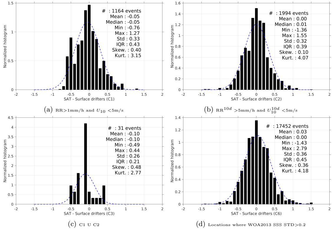
Figure 12: Normalized histogram of \Delta\text{SSS} (AQUARIUS-L2-JPL-V4 - Surface drifters) for 6 different subdatasets corresponding to: RR > 1\text{mm/h} and U_{10} < 5\text{m/s} (a), RR^{10d} > 5\text{mm/h} and U_{10}^{10d} < 5\text{m/s} (b), C1 U C2 (c), Locations where WOA2013 SSS STD > 0.2 (d).
