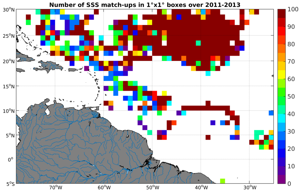
Figure 3: Number of SSS match-ups between Surface drifters SSS and the AQUARIUS-L2-JPL-V4 SSS product for the Amazon and Orinoco river plumes Pi-MEP region over 1^\circ \times 1^\circ boxes and for the full satellite product period.
