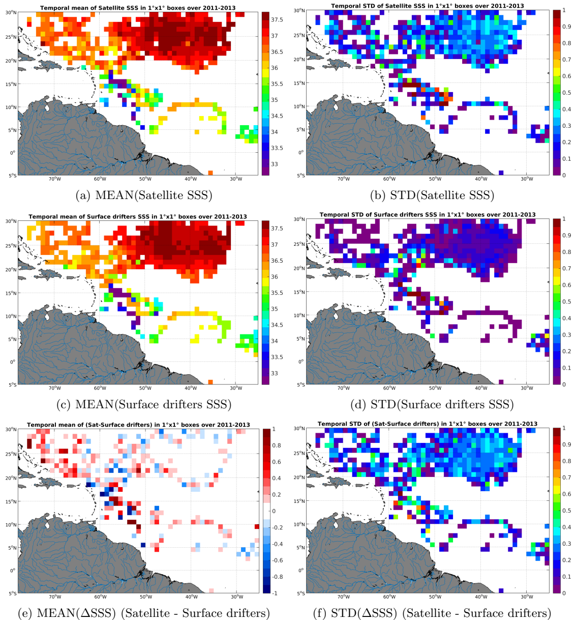
Figure 5: Temporal mean (left) and STD (right) of SSS from AQUARIUS-L2-JPL-V4 (top), Surface drifters (middle), and of \Delta SSS (Satellite - Surface drifters). Only match-up pairs are used to generate these maps.
