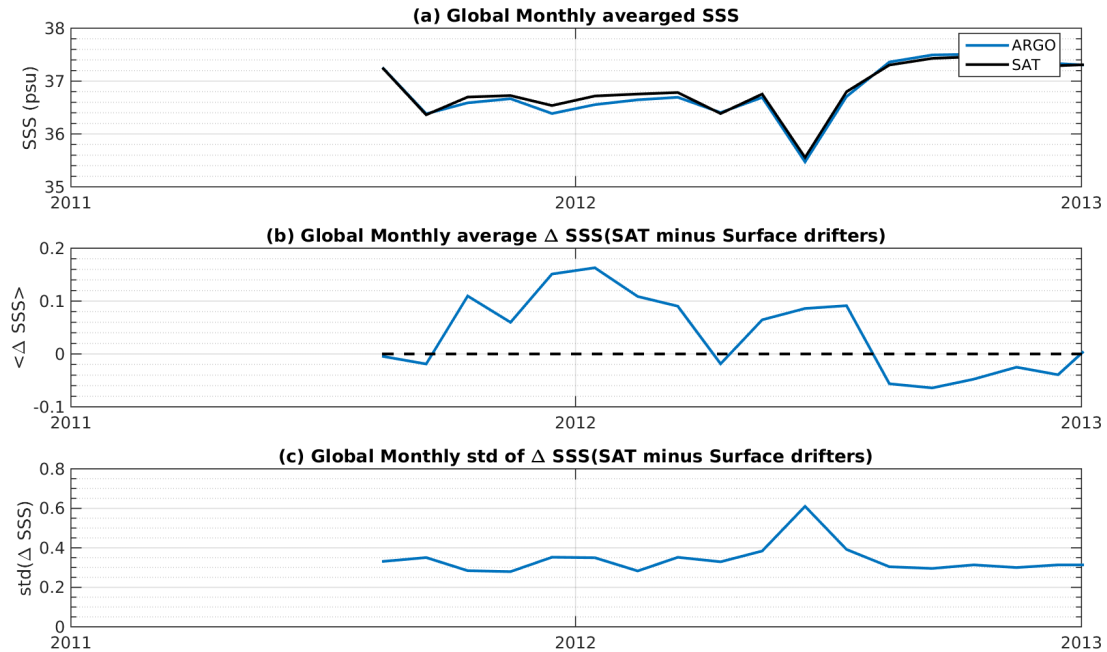
Figure 6: Time series of the monthly averaged mean SSS (top), mean \Delta SSS (Satellite - Surface drifters) and STD of \Delta SSS (Satellite - Surface drifters) over the Amazon and Orinoco river plumes Pi-MEP region considering all match-ups collected by the Pi-MEP platform.
