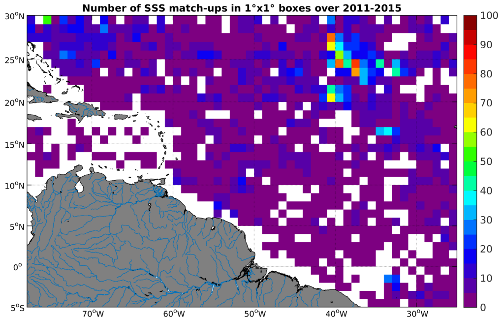
Figure 4: Number of SSS match-ups between Argo SSS and the AQUARIUS-L2-JPL-V4 SSS product for the Amazon and Orinoco river plumes Pi-MEP region over 1^\circ \times 1^\circ boxes and for the full satellite product period.
