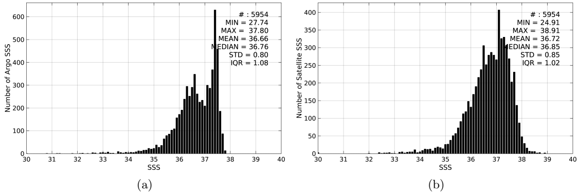
Figure 2: Histograms of SSS from Argo (a) and AQUARIUS-L2-JPL-V4 (b) considering all match-up pairs per bins of 0.1 over the Amazon and Orinoco river plumes Pi-MEP region and for the full satellite product period.
