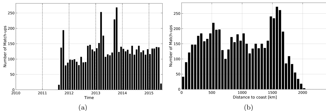
Figure 1: Number of match-ups between Argo and AQUARIUS-L2-JPL-V4 SSS as a function of time (a) and as function of the distance to coast (b) over the Amazon and Orinoco river plumes Pi-MEP region and for the full satellite product period.
