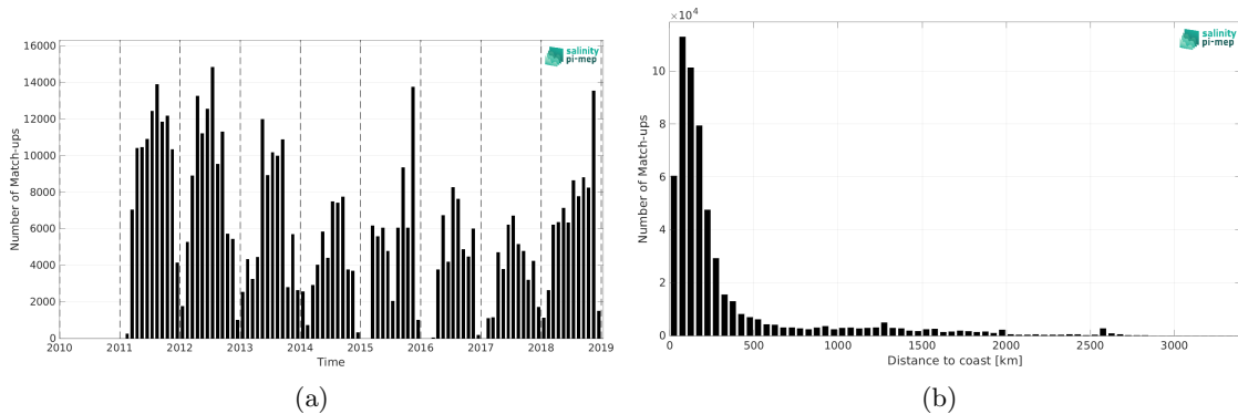
Figure 1: Number of match-ups between TSG (SAMOS) and SMOS and SMAP SSS L4 OI v1 - 7 Days (LOPS) SSS as a function of time (a) and as function of the distance to coast (b) over the Atlantic Ocean Pi-MEP region and for the full satellite product period.
