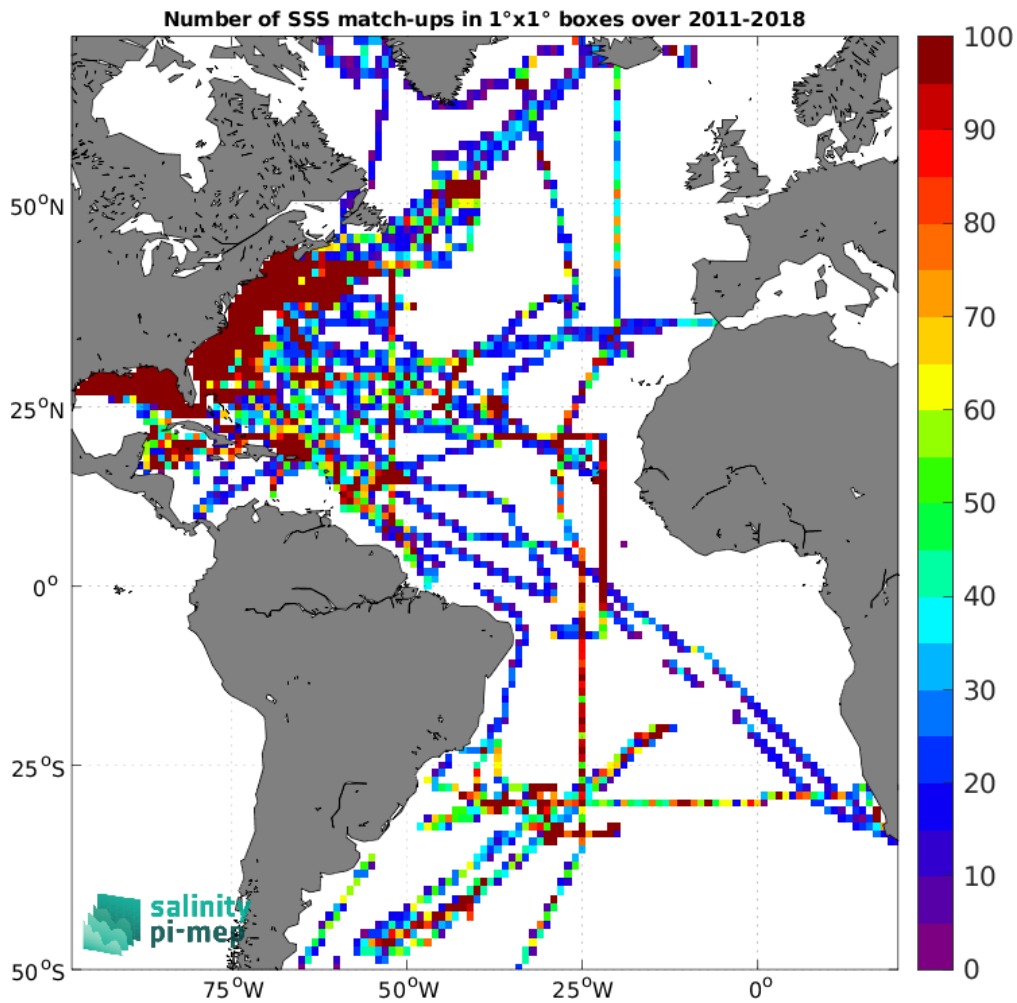
Figure 4: Number of SSS match-ups between TSG (SAMOS) SSS and the SMOS and SMAP SSS L4 OI v1 - 7 Days (LOPS) SSS product for the Atlantic Ocean Pi-MEP region over 1^\circ \times 1^\circ boxes and for the full satellite product period.
