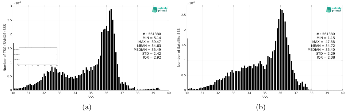
Figure 2: Histograms of SSS from TSG (SAMOS) (a) and SMOS and SMAP SSS L4 OI v1 - 7 Days (LOPS) (b) considering all match-up pairs per bins of 0.1 over the Atlantic Ocean Pi-MEP region and for the full satellite product period.
