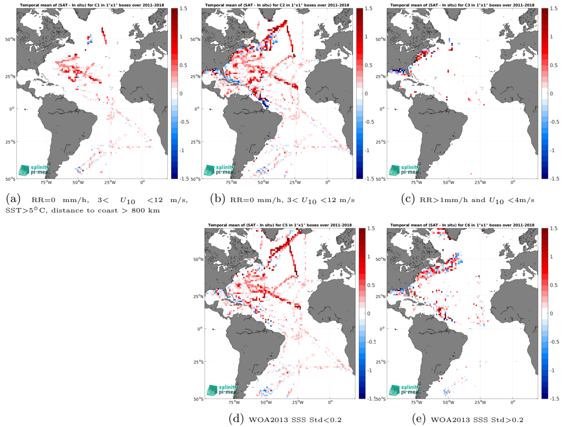
Figure 12: Temporal mean gridded over spatial boxes of size 1^\circ \times 1^\circ of \Delta SSS (SMOS and SMAP SSS L4 OI v1 - 7 Days (LOPS) - TSG (SAMOS)) for 5 different subdatasets corresponding to:RR=0 mm/h, 3 < U_{10} < 12 m/s, SST >5^\circ\text{C} , distance to coast > 800 km (a), RR=0 mm/h, 3 < U_{10} < 12 m/s (b), RR >1 mm/h and U_{10} < 4 m/s (c), WOA2013 SSS Std <0.2 (d), WOA2013 SSS Std >0.2 (e).
