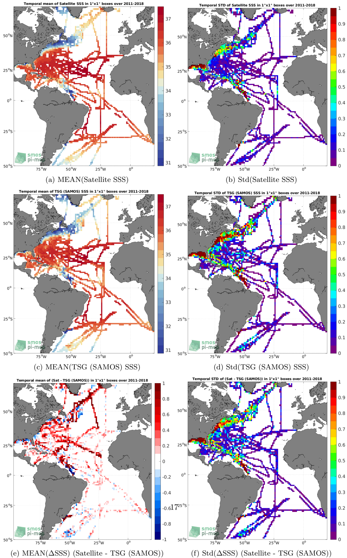
(e) MEAN( \Delta SSS) (Satellite - TSG (SAMOS)) (f) Std( \Delta SSS) (Satellite - TSG (SAMOS)) Figure 6: Temporal mean (left) and Std (right) of SSS from SMOS and SMAP SSS L4 OI v1 - 7 Days (LOPS) (top), TSG (SAMOS) (middle), and of \Delta SSS (Satellite - TSG (SAMOS)). Only match-up pairs are used to generate these maps.
