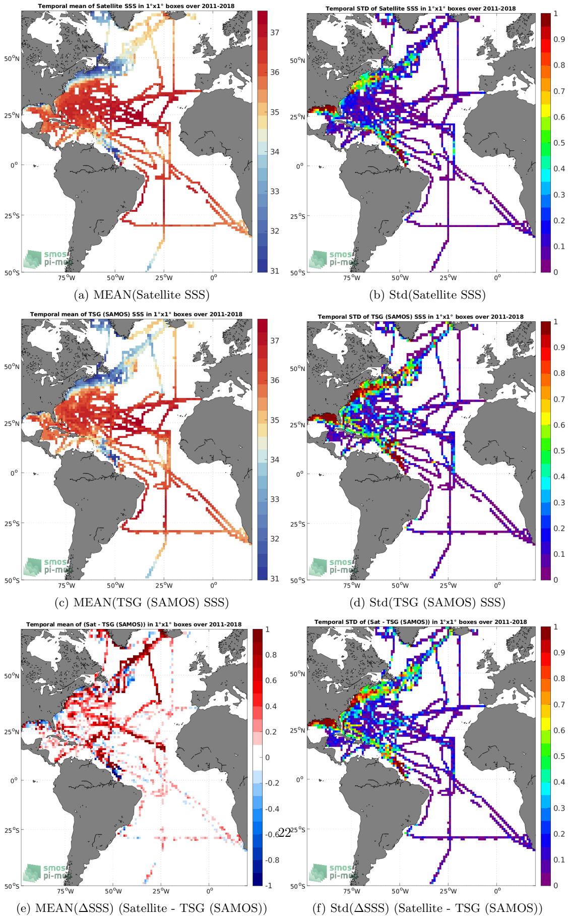
Figure 6: Temporal mean (left) and Std (right) of SSS from SMOS and SMAP SSS L4 OI v1 - 7 Days (LOPS) (top), TSG (SAMOS) (middle), and of \Delta SSS (Satellite - TSG (SAMOS)). Only match-up pairs are used to generate these maps.
