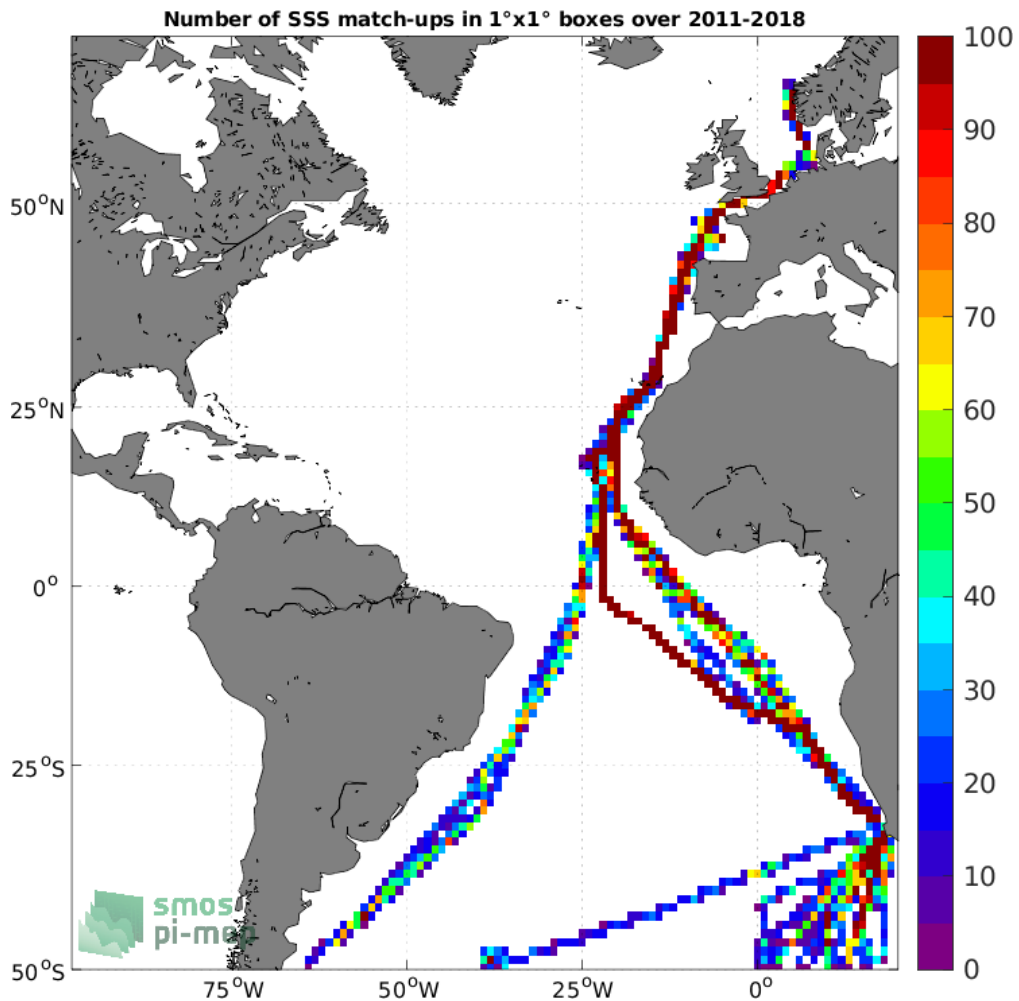
Figure 4: Number of SSS match-ups between TSG (Polarstern) SSS and the SMOS and SMAP SSS L4 OI v1 - 7 Days (LOPS) SSS product for the Atlantic Ocean Pi-MEP region over 1°x1° boxes and for the full satellite product period.
