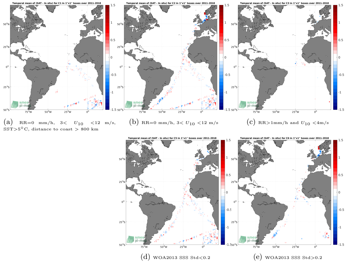
Figure 12: Temporal mean gridded over spatial boxes of size 1^\circ \times 1^\circ of \Delta SSS (SMOS and SMAP SSS L4 OI v1 - 7 Days (LOPS) - TSG (Polarstern)) for 5 different subdatasets corresponding to:RR=0 mm/h, 3 < U_{10} < 12 m/s, SST >5^\circ\text{C} , distance to coast > 800 km (a), RR=0 mm/h, 3 < U_{10} < 12 m/s (b), RR >1 mm/h and U_{10} < 4 m/s (c), WOA2013 SSS Std <0.2 (d), WOA2013 SSS Std >0.2 (e).
