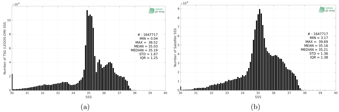
Figure 2: Histograms of SSS from TSG (LEGOS-DM) (a) and SMOS and SMAP SSS L4 OI v1 - 7 Days (LOPS) (b) considering all match-up pairs per bins of 0.1 over the Atlantic Ocean Pi-MEP region and for the full satellite product period.
