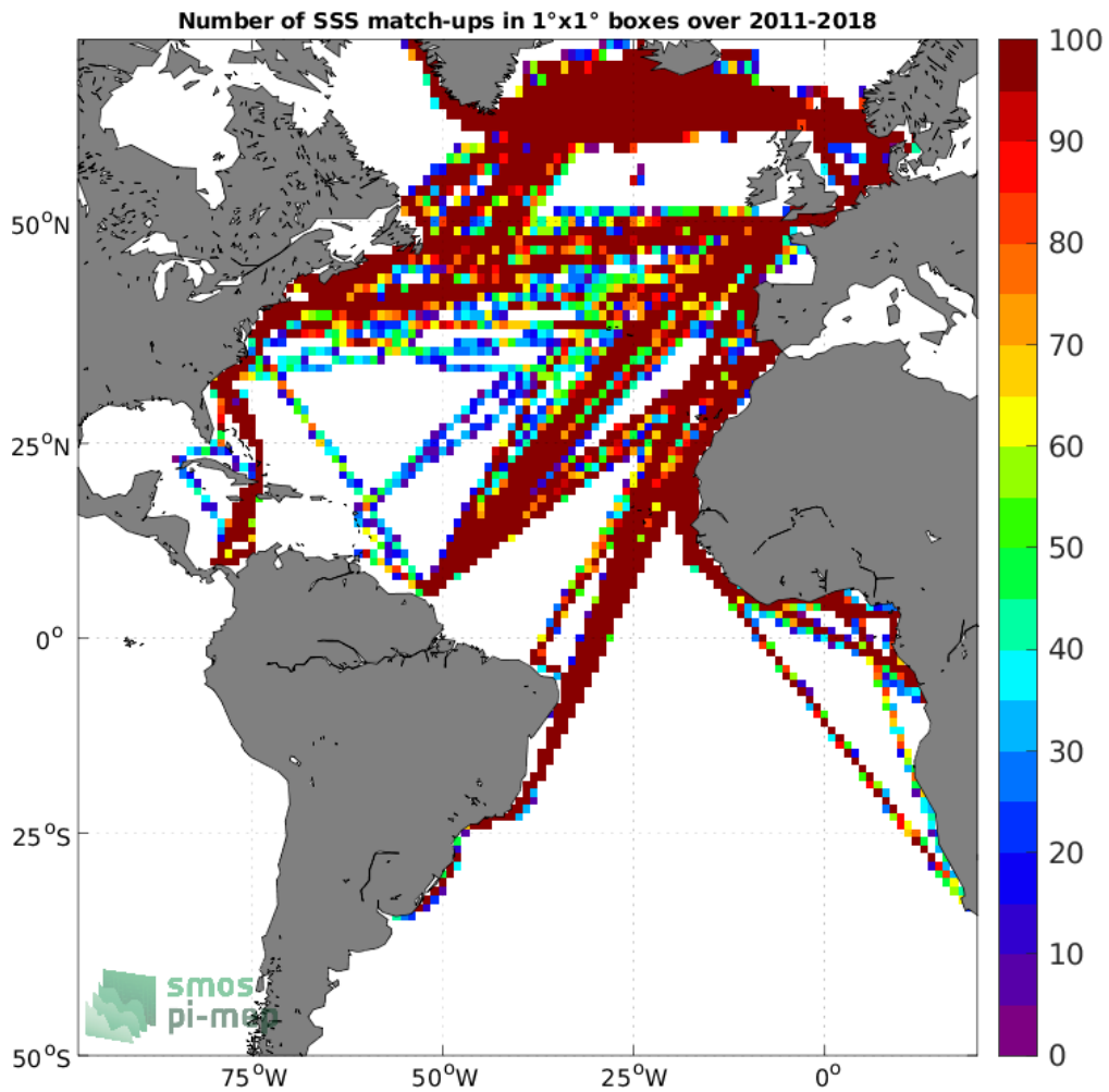
Figure 4: Number of SSS match-ups between TSG (LEGOS-DM) SSS and the SMOS and SMAP SSS L4 OI v1 - 7 Days (LOPS) SSS product for the Atlantic Ocean Pi-MEP region over 1°x1° boxes and for the full satellite product period.
