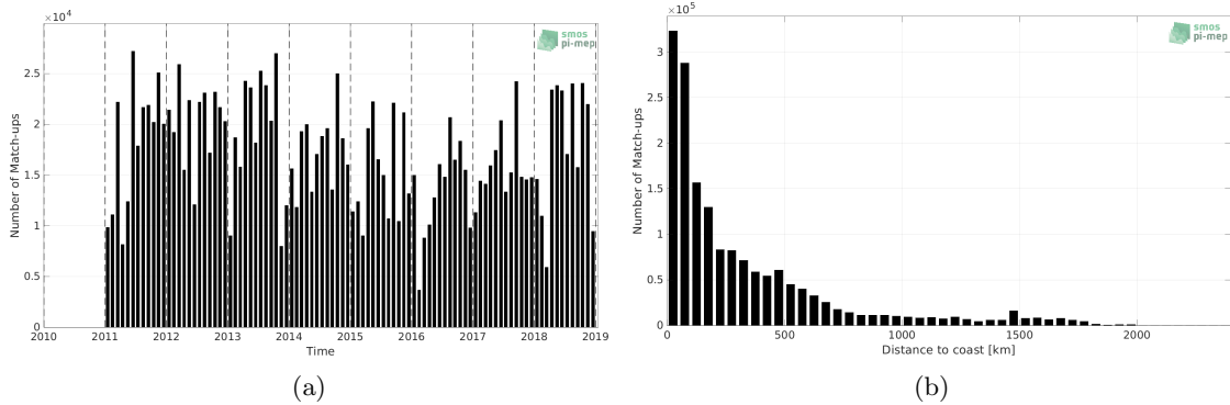
Figure 1: Number of match-ups between TSG (LEGOS-DM) and SMOS and SMAP SSS L4 OI v1 - 7 Days (LOPS) SSS as a function of time (a) and as function of the distance to coast (b) over the Atlantic Ocean Pi-MEP region and for the full satellite product period.
