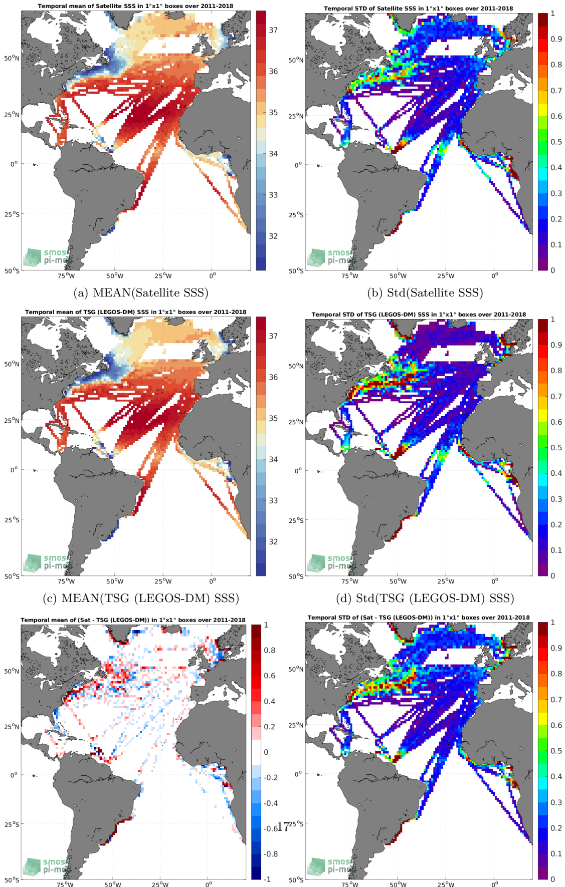
(e) MEAN( \Delta SSS) (Satellite - TSG (LEGOS-DM)) (f) Std( \Delta SSS) (Satellite - TSG (LEGOS-DM)) Figure 6: Temporal mean (left) and Std (right) of SSS from SMOS and SMAP SSS L4 OI v1 - 7 Days (LOPS) (top), TSG (LEGOS-DM) (middle), and of \Delta SSS (Satellite - TSG (LEGOS-DM)). Only match-up pairs are used to generate these maps.
