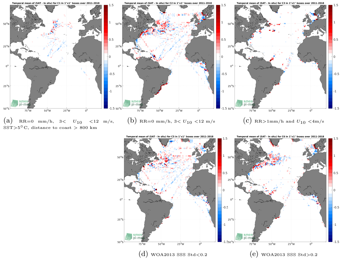
Figure 12: Temporal mean gridded over spatial boxes of size 1^\circ \times 1^\circ of \Delta\text{SSS} (SMOS and SMAP SSS L4 OI v1 - 7 Days (LOPS) - TSG (LEGOS-DM)) for 5 different subdatasets corresponding to:RR=0 mm/h, 3 < U_{10} < 12 m/s, SST >5^\circ\text{C} , distance to coast > 800 km (a), RR=0 mm/h, 3 < U_{10} < 12 m/s (b), RR >1 mm/h and U_{10} < 4 m/s (c), WOA2013 SSS Std <0.2 (d), WOA2013 SSS Std >0.2 (e).
