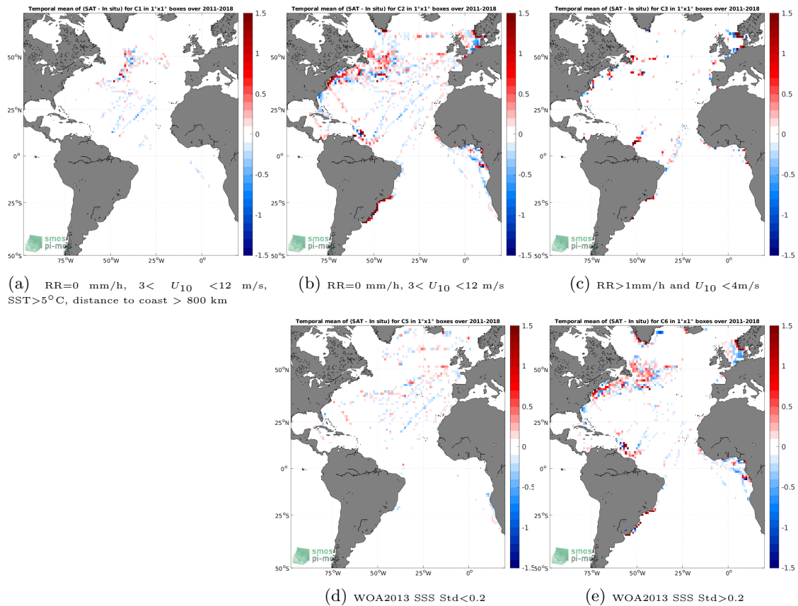
Figure 12: Temporal mean gridded over spatial boxes of size 1^\circ \times 1^\circ of \Delta SSS (SMOS and SMAP SSS L4 OI v1 - 7 Days (LOPS) - TSG (LEGOS-DM)) for 5 different subdatasets corresponding to:RR=0 mm/h, 3 < U_{10} < 12 m/s, SST >5^\circ\text{C} , distance to coast > 800 km (a), RR=0 mm/h, 3 < U_{10} < 12 m/s (b), RR >1 mm/h and U_{10} < 4 m/s (c), WOA2013 SSS Std <0.2 (d), WOA2013 SSS Std >0.2 (e).
