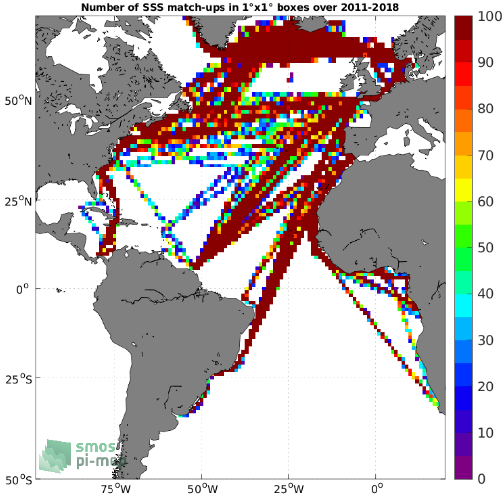
Figure 4: Number of SSS match-ups between TSG (LEGOS-DM) SSS and the SMOS and SMAP SSS L4 OI v1 - 7 Days (LOPS) SSS product for the Atlantic Ocean Pi-MEP region over 1^\circ \times 1^\circ boxes and for the full satellite product period.
