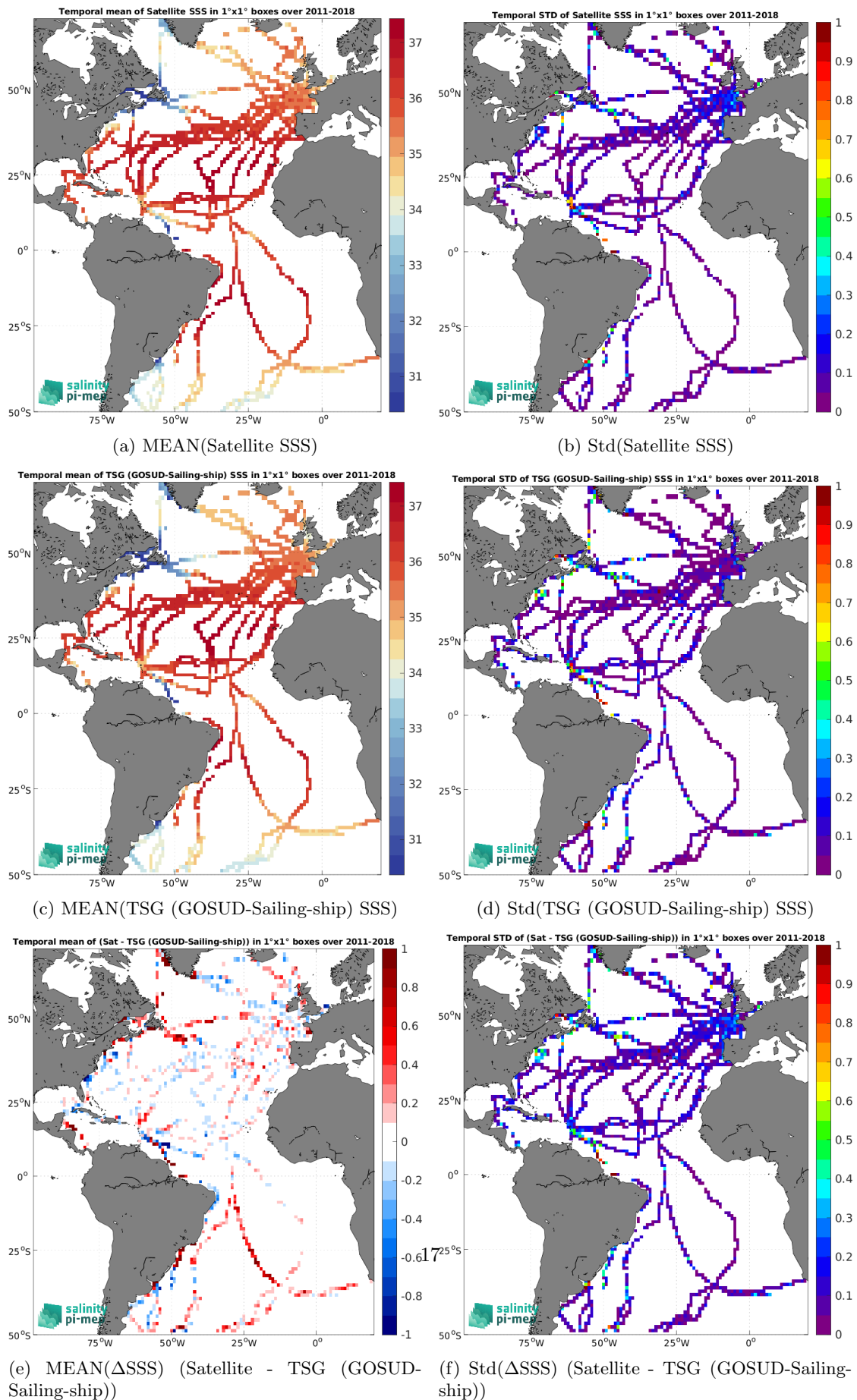
Figure 6: Temporal mean (left) and Std (right) of SSS from SMOS and SMAP SSS L4 OI v1 - 7 Days (LOPS) (top), TSG (GOSUD-Sailing-ship) (middle), and of \Delta\text{SSS} (Satellite - TSG (GOSUD-Sailing-ship)). Only match-up pairs are used to generate these maps.
