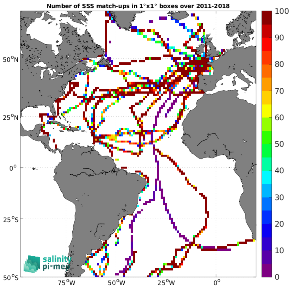
Figure 4: Number of SSS match-ups between TSG (GOSUD-Sailing-ship) SSS and the SMOS and SMAP SSS L4 OI v1 - 7 Days (LOPS) SSS product for the Atlantic Ocean Pi-MEP region over 1°x1° boxes and for the full satellite product period.
