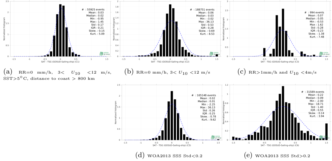
Figure 13: Normalized histogram of \Delta\text{SSS} (SMOS and SMAP SSS L4 OI v1 - 7 Days (LOPS) - TSG (GOSUD-Sailing-ship)) for 5 different subdatasets corresponding to: RR=0 mm/h, 3 < U_{10} < 12 m/s, SST>5°C, distance to coast > 800 km (a), RR=0 mm/h, 3 < U_{10} < 12 m/s (b), RR>1mm/h and U_{10} < 4 m/s (c), WOA2013 SSS Std<0.2 (d), WOA2013 SSS Std>0.2 (e).
