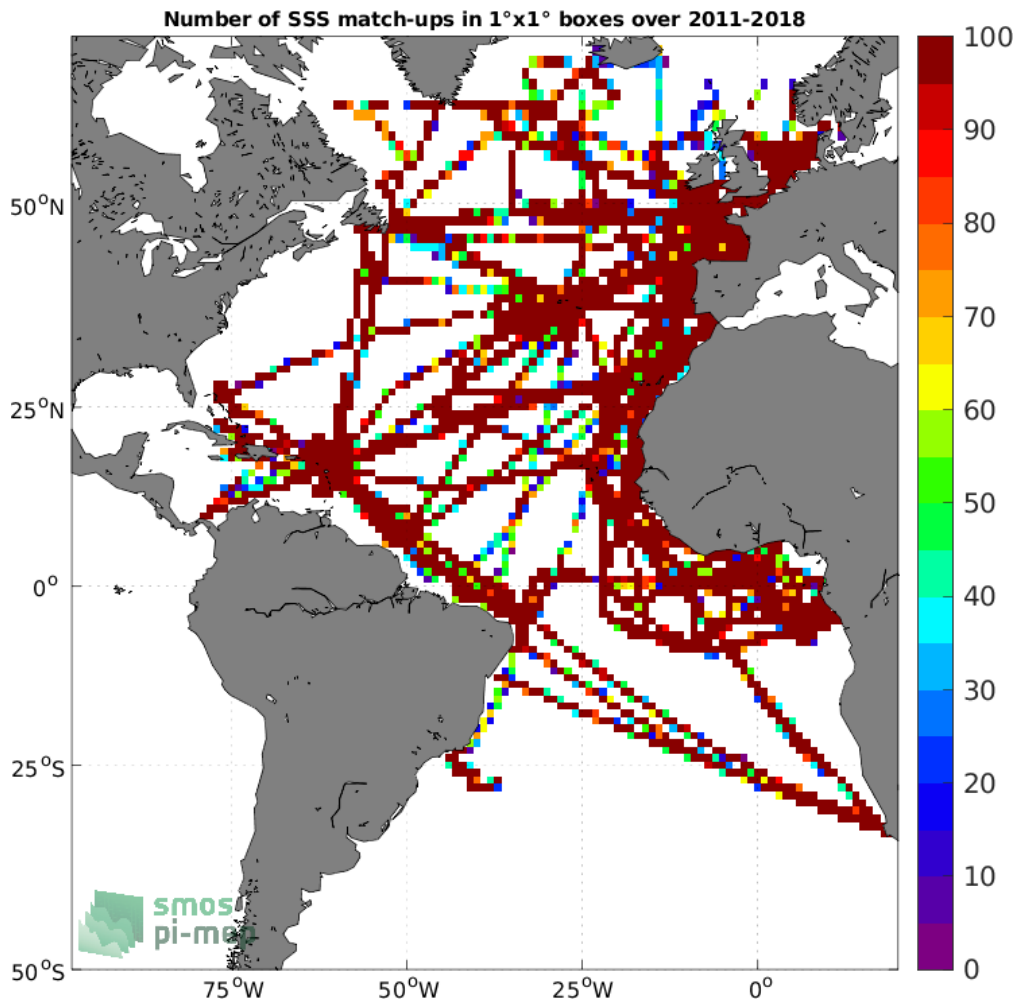
Figure 4: Number of SSS match-ups between TSG (GOSUD-Research-vessel) SSS and the SMOS and SMAP SSS L4 OI v1 - 7 Days (LOPS) SSS product for the Atlantic Ocean Pi-MEP region over 1°x1° boxes and for the full satellite product period.
