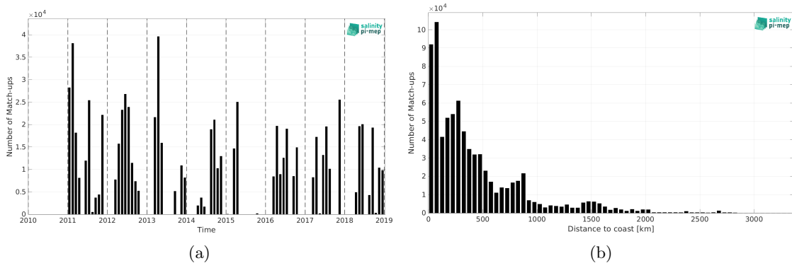
Figure 1: Number of match-ups between TSG (CSIC-UTM) and SMOS and SMAP SSS L4 OI v1 - 7 Days (LOPS) SSS as a function of time (a) and as function of the distance to coast (b) over the Atlantic Ocean Pi-MEP region and for the full satellite product period.
