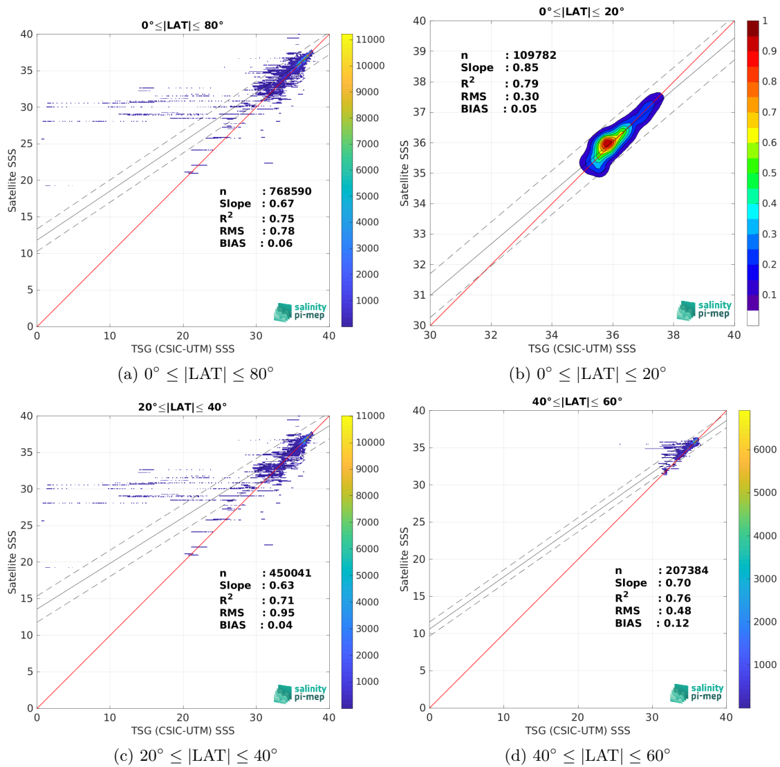
Figure 9: Contour maps of the concentration of SMOS and SMAP SSS L4 OI v1 - 7 Days (LOPS) SSS (y-axis) versus TSG (CSIC-UTM) SSS (x-axis) at match-up pairs for different latitude bands. For each plot, the red line shows x=y . The black thin and dashed lines indicate a linear fit through the data cloud and the \pm 95\% confidence levels, respectively. The number match-up pairs n , the slope and R^2 coefficient of the linear fit, the root mean square (RMS) and the mean bias between satellite and in situ data are indicated for each latitude band in each plots.
