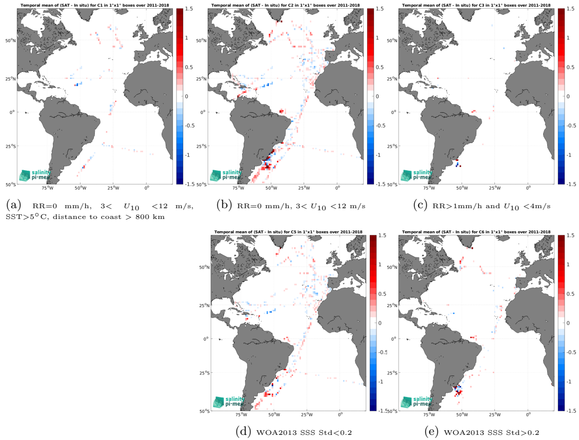
Figure 12: Temporal mean gridded over spatial boxes of size 1^\circ \times 1^\circ of \Delta SSS (SMOS and SMAP SSS L4 OI v1 - 7 Days (LOPS) - TSG (CSIC-UTM)) for 5 different subdatasets corresponding to:RR=0 mm/h, 3 < U_{10} < 12 m/s, SST >5^\circ\text{C} , distance to coast > 800 km (a), RR=0 mm/h, 3 < U_{10} < 12 m/s (b), RR >1 mm/h and U_{10} < 4 m/s (c), WOA2013 SSS Std <0.2 (d), WOA2013 SSS Std >0.2 (e).
