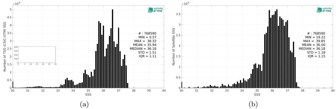
Figure 2: Histograms of SSS from TSG (CSIC-UTM) (a) and SMOS and SMAP SSS L4 OI v1 - 7 Days (LOPS) (b) considering all match-up pairs per bins of 0.1 over the Atlantic Ocean Pi-MEP region and for the full satellite product period.
