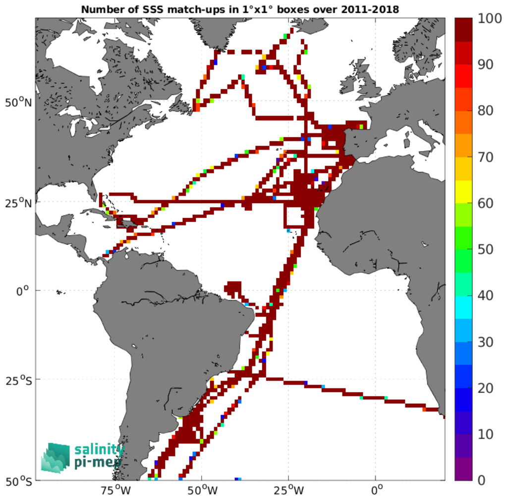
Figure 4: Number of SSS match-ups between TSG (CSIC-UTM) SSS and the SMOS and SMAP SSS L4 OI v1 - 7 Days (LOPS) SSS product for the Atlantic Ocean Pi-MEP region over 1°x1° boxes and for the full satellite product period.
