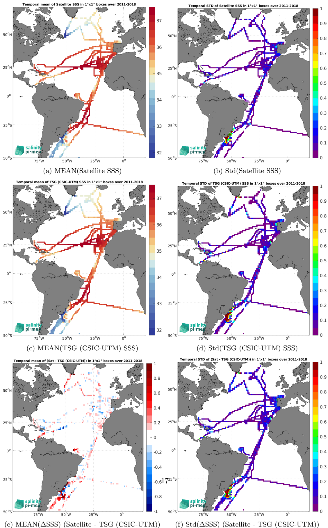
Figure 6: Temporal mean (left) and Std (right) of SSS from SMOS and SMAP SSS L4 OI v1 - 7 Days (LOPS) (top), TSG (CSIC-UTM) (middle), and of \Delta SSS (Satellite - TSG (CSIC-UTM)). Only match-up pairs are used to generate these maps.
