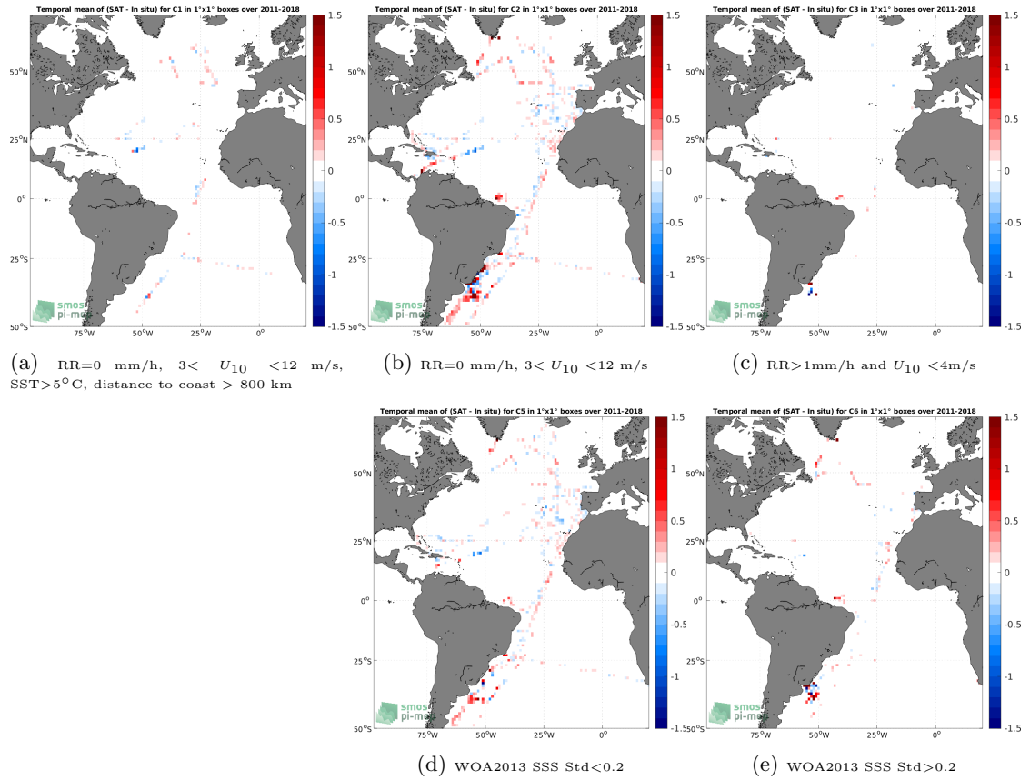
Figure 12: Temporal mean gridded over spatial boxes of size 1^\circ \times 1^\circ of \Delta SSS (SMOS and SMAP SSS L4 OI v1 - 7 Days (LOPS) - TSG (CSIC-UTM)) for 5 different subdatasets corresponding to:RR=0 mm/h, 3 < U_{10} < 12 m/s, SST >5^\circ\text{C} , distance to coast > 800 km (a), RR=0 mm/h, 3 < U_{10} < 12 m/s (b), RR >1 mm/h and U_{10} < 4 m/s (c), WOA2013 SSS Std <0.2 (d), WOA2013 SSS Std >0.2 (e).
