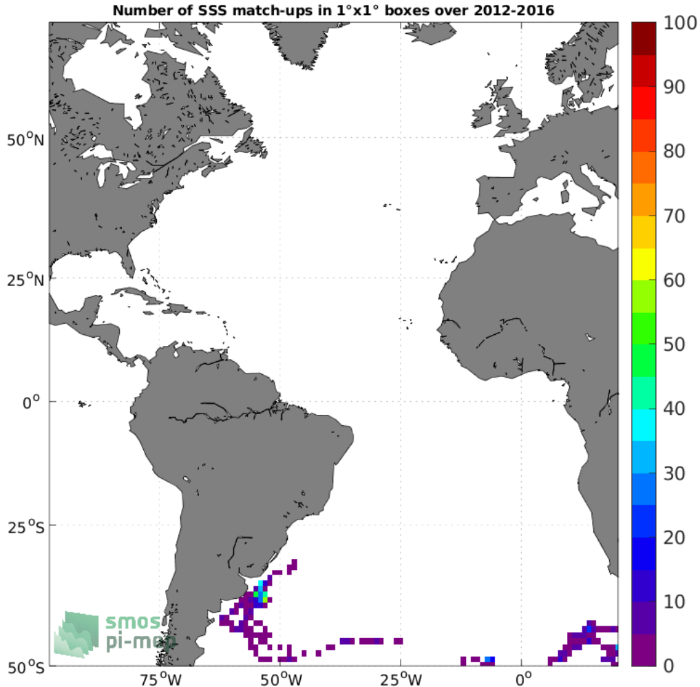
Figure 4: Number of SSS match-ups between Marine mammals SSS and the SMOS and SMAP SSS L4 OI v1 - 7 Days (LOPS) SSS product for the Atlantic Ocean Pi-MEP region over 1^\circ \times 1^\circ boxes and for the full satellite product period.
