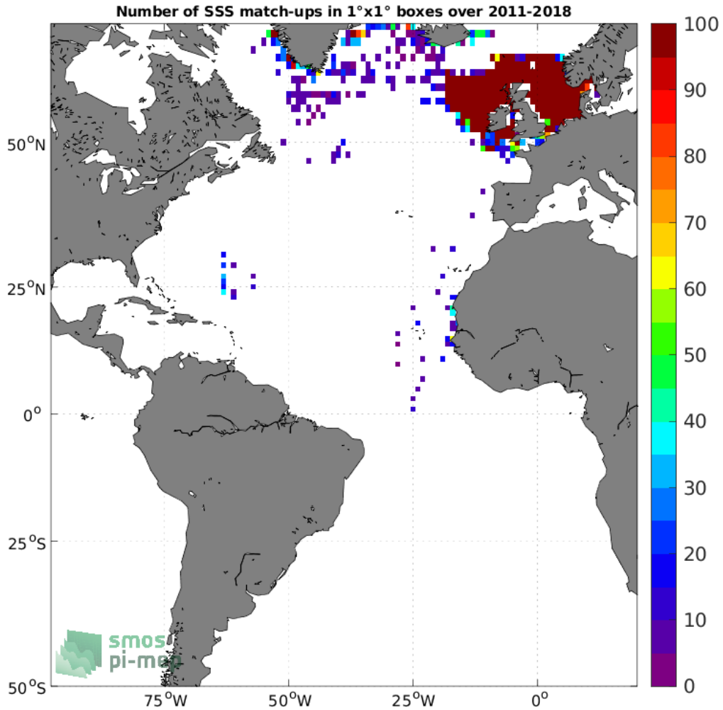
Figure 4: Number of SSS match-ups between ICES SSS and the SMOS and SMAP SSS L4 OI v1 - 7 Days (LOPS) SSS product for the Atlantic Ocean Pi-MEP region over 1^\circ \times 1^\circ boxes and for the full satellite product period.
