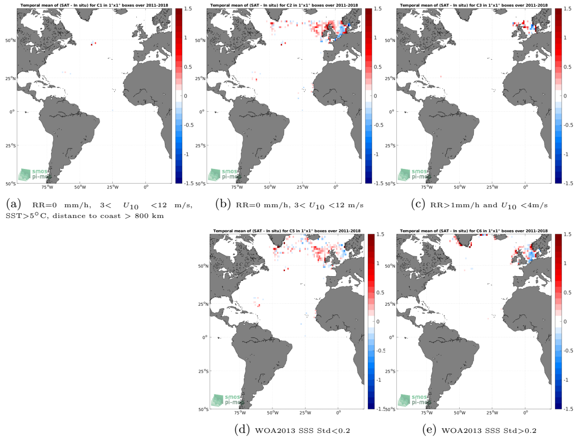
Figure 12: Temporal mean gridded over spatial boxes of size 1^\circ \times 1^\circ of \Delta SSS (SMOS and SMAP SSS L4 OI v1 - 7 Days (LOPS) - ICES) for 5 different subdatasets corresponding to:RR=0 mm/h, 3 < U_{10} < 12 m/s, SST >5^\circ\text{C} , distance to coast > 800 km (a), RR=0 mm/h, 3 < U_{10} < 12 m/s (b), RR >1 mm/h and U_{10} < 4 m/s (c), WOA2013 SSS Std <0.2 (d), WOA2013 SSS Std >0.2 (e).
