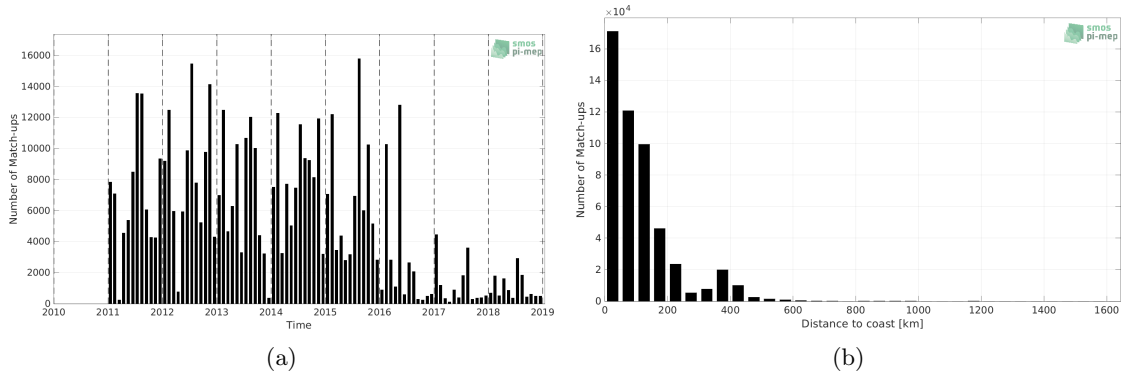
Figure 1: Number of match-ups between ICES and SMOS and SMAP SSS L4 OI v1 - 7 Days (LOPS) SSS as a function of time (a) and as function of the distance to coast (b) over the Atlantic Ocean Pi-MEP region and for the full satellite product period.
