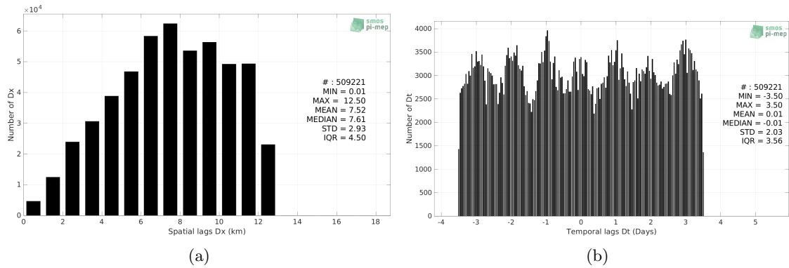
Figure 5: Histograms of the spatial (a) and temporal (b) lags between the location/time of the ICES measurement and the date of the corresponding SMOS and SMAP SSS L4 OI v1 - 7 Days (LOPS) SSS pixel.
