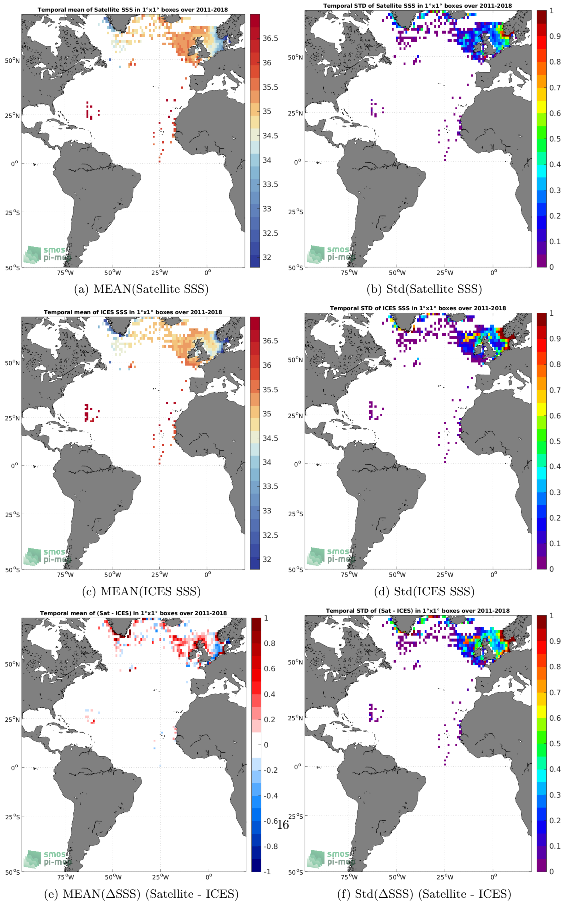
Figure 6: Temporal mean (left) and Std (right) of SSS from SMOS and SMAP SSS L4 OI v1 - 7 Days (LOPS) (top), ICES (middle), and of \Delta SSS (Satellite - ICES). Only match-up pairs are used to generate these maps.
