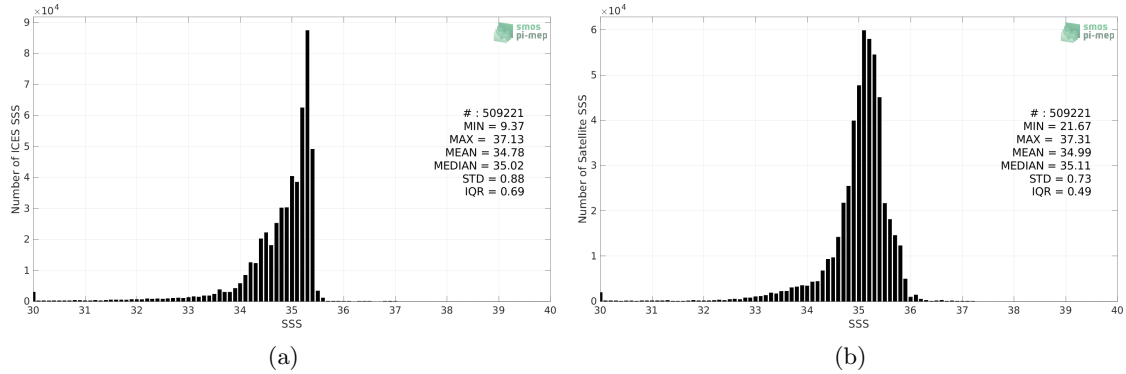
Figure 2: Histograms of SSS from ICES (a) and SMOS and SMAP SSS L4 OI v1 - 7 Days (LOPS) (b) considering all match-up pairs per bins of 0.1 over the Atlantic Ocean Pi-MEP region and for the full satellite product period.
