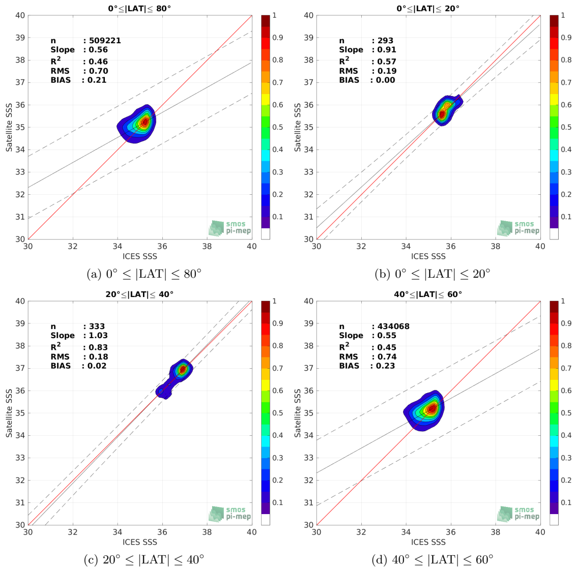
Figure 9: Contour maps of the concentration of SMOS and SMAP SSS L4 OI v1 - 7 Days (LOPS) SSS (y-axis) versus ICES SSS (x-axis) at match-up pairs for different latitude bands. For each plot, the red line shows x=y . The black thin and dashed lines indicate a linear fit through the data cloud and the \pm 95\% confidence levels, respectively. The number match-up pairs n , the slope and R^2 coefficient of the linear fit, the root mean square (RMS) and the mean bias between satellite and in situ data are indicated for each latitude band in each plots.
