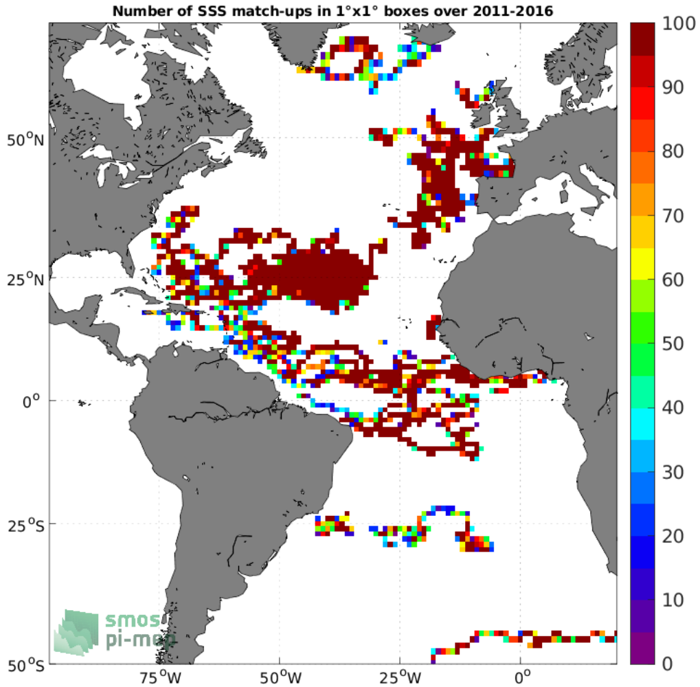
Figure 3: Number of SSS match-ups between Surface drifters SSS and the SMOS and SMAP SSS L4 OI v1 - 7 Days (LOPS) SSS product for the Atlantic Ocean Pi-MEP region over 1^\circ \times 1^\circ boxes and for the full satellite product period.
