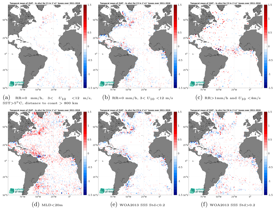
Figure 12: Temporal mean gridded over spatial boxes of size 1^\circ \times 1^\circ of \Delta SSS (SMOS and SMAP SSS L4 OI v1 - 7 Days (LOPS) - Argo) for 6 different subdatasets corresponding to:RR=0 mm/h, 3 < U_{10} < 12 m/s, SST > 5^\circ\text{C} , distance to coast > 800 km (a), RR=0 mm/h, 3 < U_{10} < 12 m/s (b), RR > 1 mm/h and U_{10} < 4 m/s (c),MLD < 20 m (d),WOA2013 SSS Std < 0.2 (e),WOA2013 SSS Std > 0.2 (f).
