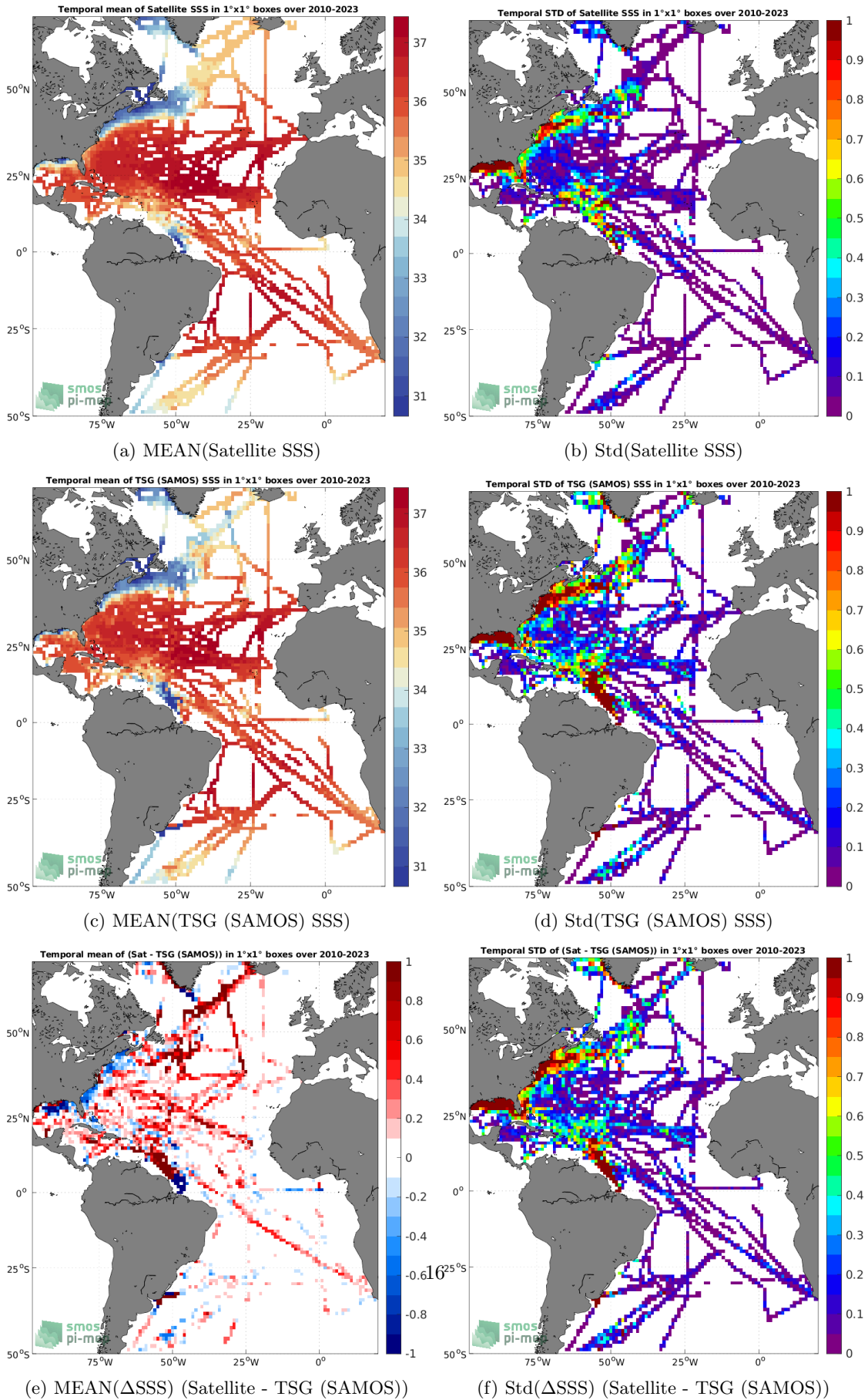
Figure 6: Temporal mean (left) and Std (right) of SSS from SMOS SSS L4 v1 - Weekly (CMEMS-CNR) (top), TSG (SAMOS) (middle), and of \Delta SSS (Satellite - TSG (SAMOS)). Only match-up pairs are used to generate these maps.
