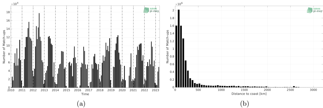
Figure 1: Number of match-ups between TSG (SAMOS) and SMOS SSS L4 v1 - Weekly (CMEMS-CNR) SSS as a function of time (a) and as function of the distance to coast (b) over the Atlantic Ocean Pi-MEP region and for the full satellite product period.
