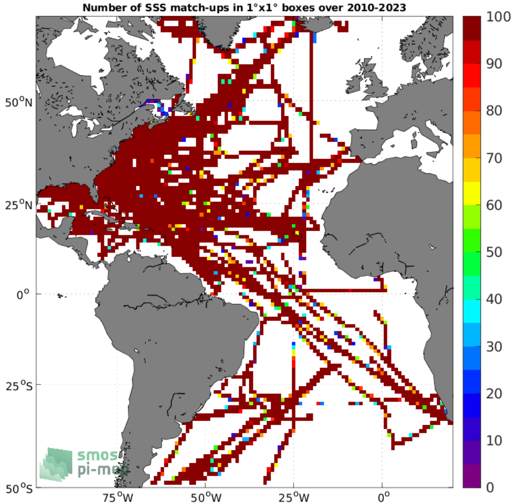
Figure 4: Number of SSS match-ups between TSG (SAMOS) SSS and the SMOS SSS L4 v1 - Weekly (CMEMS-CNR) SSS product for the Atlantic Ocean Pi-MEP region over 1^\circ \times 1^\circ boxes and for the full satellite product period.
