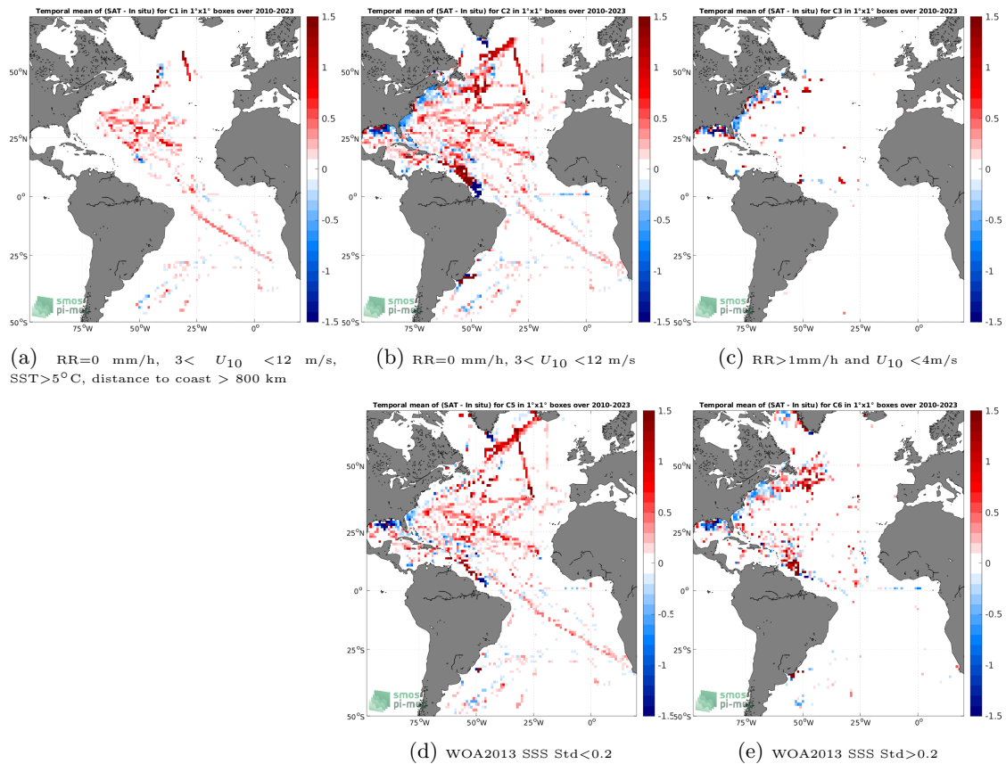
Figure 12: Temporal mean gridded over spatial boxes of size 1^\circ \times 1^\circ of \Delta SSS (SMOS SSS L4 v1 - Weekly (CMEMS-CNR) - TSG (SAMOS)) for 5 different subdatasets corresponding to:RR=0 mm/h, 3 < U_{10} < 12 m/s, SST >5^\circ\text{C} , distance to coast > 800 km (a), RR=0 mm/h, 3 < U_{10} < 12 m/s (b), RR >1 mm/h and U_{10} < 4 m/s (c), WOA2013 SSS Std <0.2 (d), WOA2013 SSS Std >0.2 (e).
