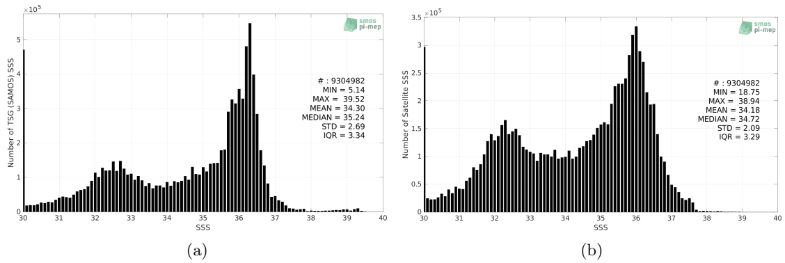
Figure 2: Histograms of SSS from TSG (SAMOS) (a) and SMOS SSS L4 v1 - Weekly (CMEMS-CNR) (b) considering all match-up pairs per bins of 0.1 over the Atlantic Ocean Pi-MEP region and for the full satellite product period.
