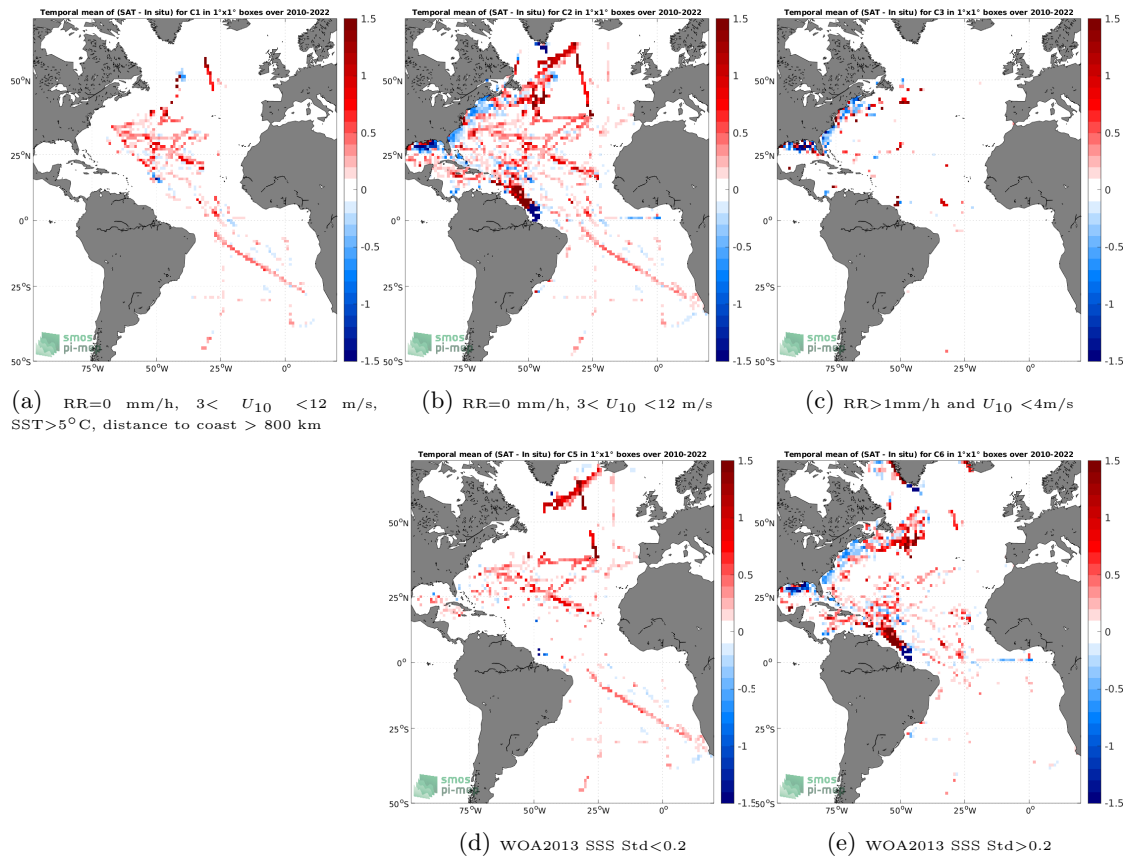
Figure 12: Temporal mean gridded over spatial boxes of size 1^\circ \times 1^\circ of \Delta\text{SSS} (SMOS SSS L4 v1 - Weekly (CMEMS-CNR) - TSG (SAMOS)) for 5 different subdatasets corresponding to:RR=0 mm/h, 3 < U_{10} < 12 m/s, SST >5^\circ\text{C} , distance to coast > 800 km (a), RR=0 mm/h, 3 < U_{10} < 12 m/s (b), RR >1 mm/h and U_{10} < 4 m/s (c), WOA2013 SSS Std <0.2 (d), WOA2013 SSS Std >0.2 (e).
