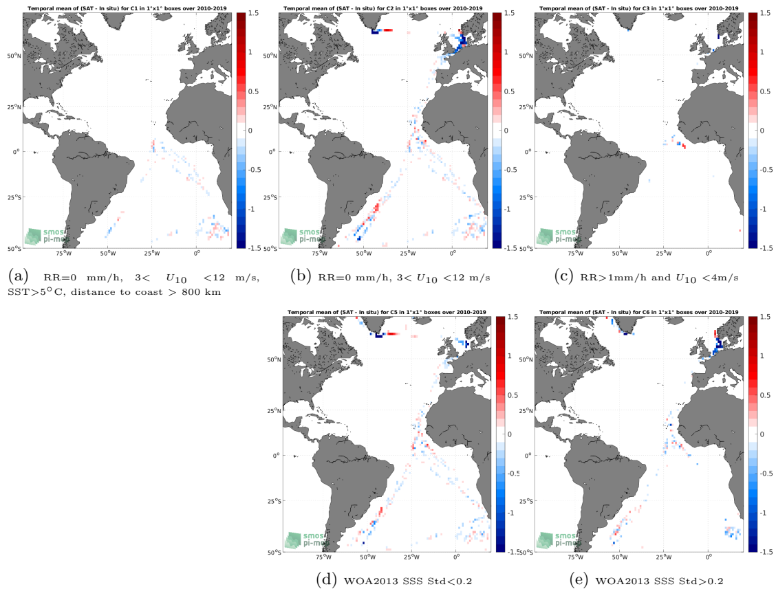
Figure 12: Temporal mean gridded over spatial boxes of size 1^\circ \times 1^\circ of \Delta\text{SSS} (SMOS SSS L4 v1 - Weekly (CMEMS-CNR) - TSG (Polarstern)) for 5 different subdatasets corresponding to:RR=0 mm/h, 3 < U_{10} < 12 m/s, SST >5^\circ\text{C} , distance to coast > 800 km (a), RR=0 mm/h, 3 < U_{10} < 12 m/s (b), RR >1 mm/h and U_{10} < 4 m/s (c), WOA2013 SSS Std <0.2 (d), WOA2013 SSS Std >0.2 (e).
