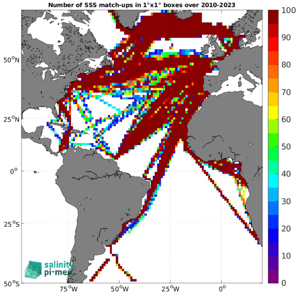
Figure 4: Number of SSS match-ups between TSG (LEGOS-DM) SSS and the SMOS SSS L4 v1 - Weekly (CMEMS-CNR) SSS product for the Atlantic Ocean Pi-MEP region over 1^\circ \times 1^\circ boxes and for the full satellite product period.
