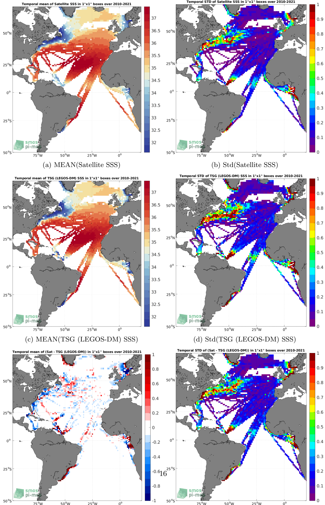
(e) MEAN( \Delta SSS) (Satellite - TSG (LEGOS-DM)) (f) Std( \Delta SSS) (Satellite - TSG (LEGOS-DM)) Figure 6: Temporal mean (left) and Std (right) of SSS from SMOS SSS L4 v1 - Weekly (CMEMS-CNR) (top), TSG (LEGOS-DM) (middle), and of \Delta SSS (Satellite - TSG (LEGOS-DM)). Only match-up pairs are used to generate these maps.
