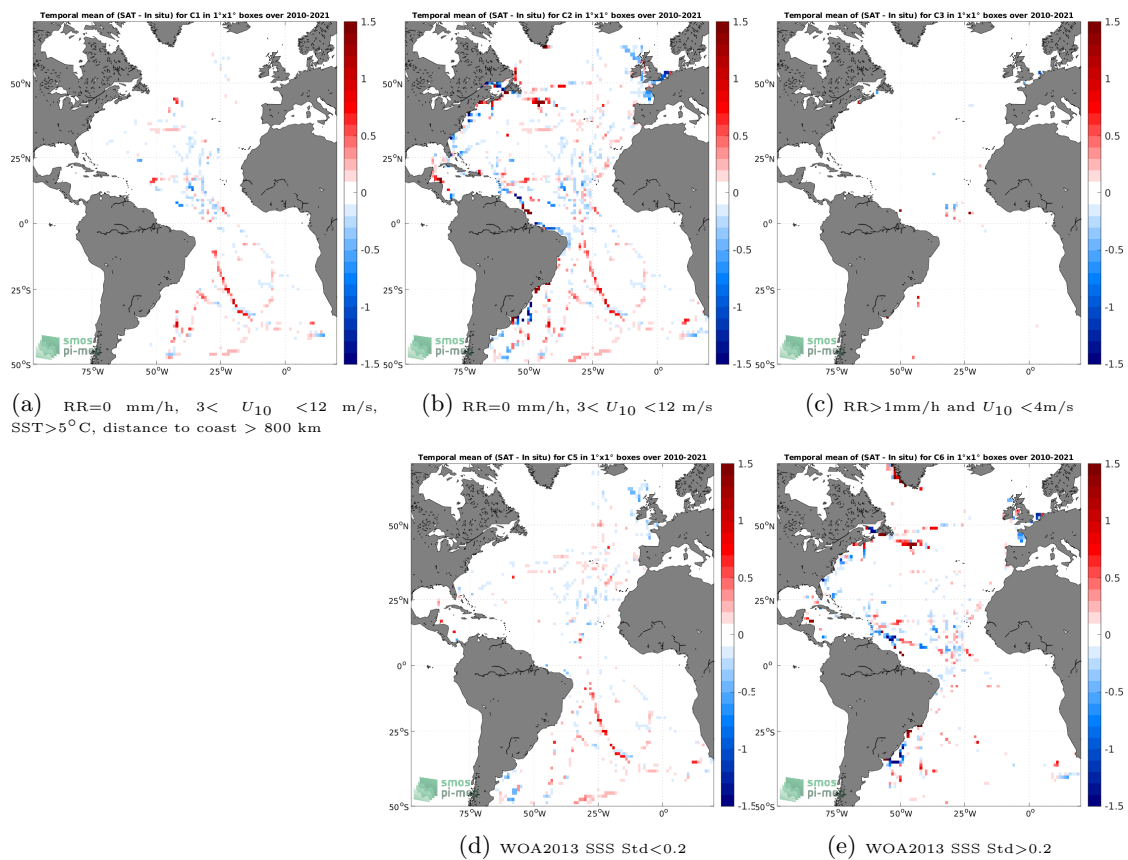
Figure 12: Temporal mean gridded over spatial boxes of size 1^\circ \times 1^\circ of \Delta\text{SSS} (SMOS SSS L4 v1 - Weekly (CMEMS-CNR) - TSG (GOSUD-Sailing-ship)) for 5 different subdatasets corresponding to:RR=0 mm/h, 3 < U_{10} < 12 m/s, SST>5°C, distance to coast > 800 km (a), RR=0 mm/h, 3 < U_{10} < 12 m/s (b), RR>1mm/h and U_{10} < 4 m/s (c), WOA2013 SSS Std<0.2 (d), WOA2013 SSS Std>0.2 (e).
