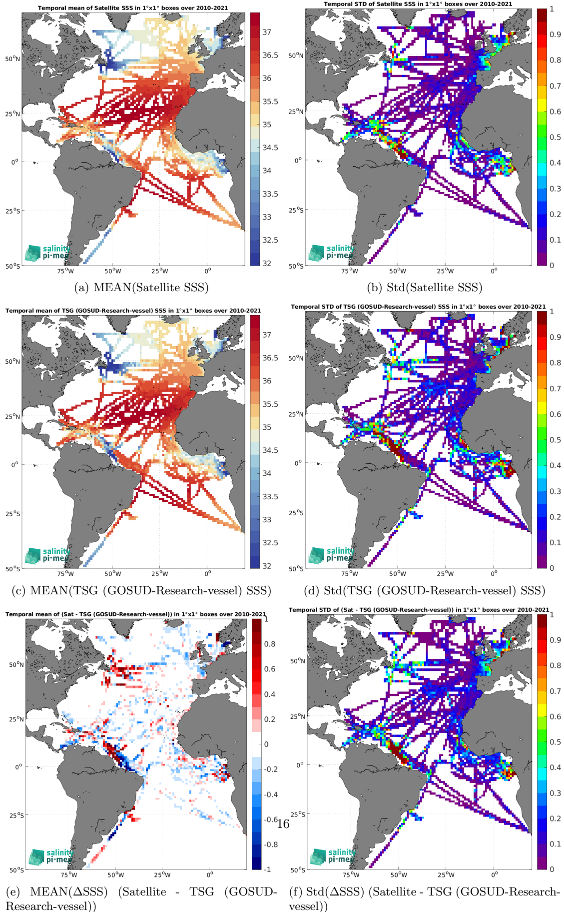
Figure 6: Temporal mean (left) and Std (right) of SSS from SMOS SSS L4 v1 - Weekly (CMEMS-CNR) (top), TSG (GOSUD-Research-vessel) (middle), and of \Delta SSS (Satellite - TSG (GOSUD-Research-vessel)). Only match-up pairs are used to generate these maps.
