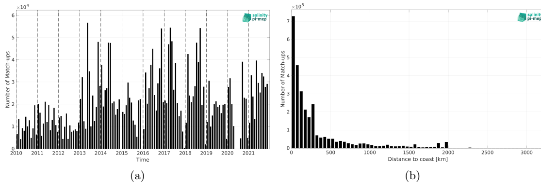
Figure 1: Number of match-ups between TSG (GOSUD-Research-vessel) and SMOS SSS L4 v1 - Weekly (CMEMS-CNR) SSS as a function of time (a) and as function of the distance to coast (b) over the Atlantic Ocean Pi-MEP region and for the full satellite product period.
