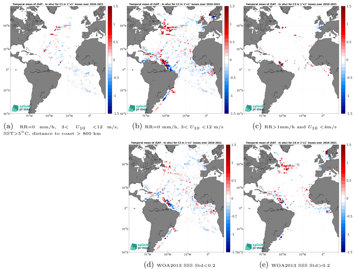
Figure 12: Temporal mean gridded over spatial boxes of size 1^\circ \times 1^\circ of \Delta SSS (SMOS SSS L4 v1 - Weekly (CMEMS-CNR) - TSG (GOSUD-Research-vessel)) for 5 different subdatasets corresponding to:RR=0 mm/h, 3 < U_{10} < 12 m/s, SST>5°C, distance to coast > 800 km (a), RR=0 mm/h, 3 < U_{10} < 12 m/s (b), RR>1mm/h and U_{10} < 4 m/s (c), WOA2013 SSS Std<0.2 (d), WOA2013 SSS Std>0.2 (e).
