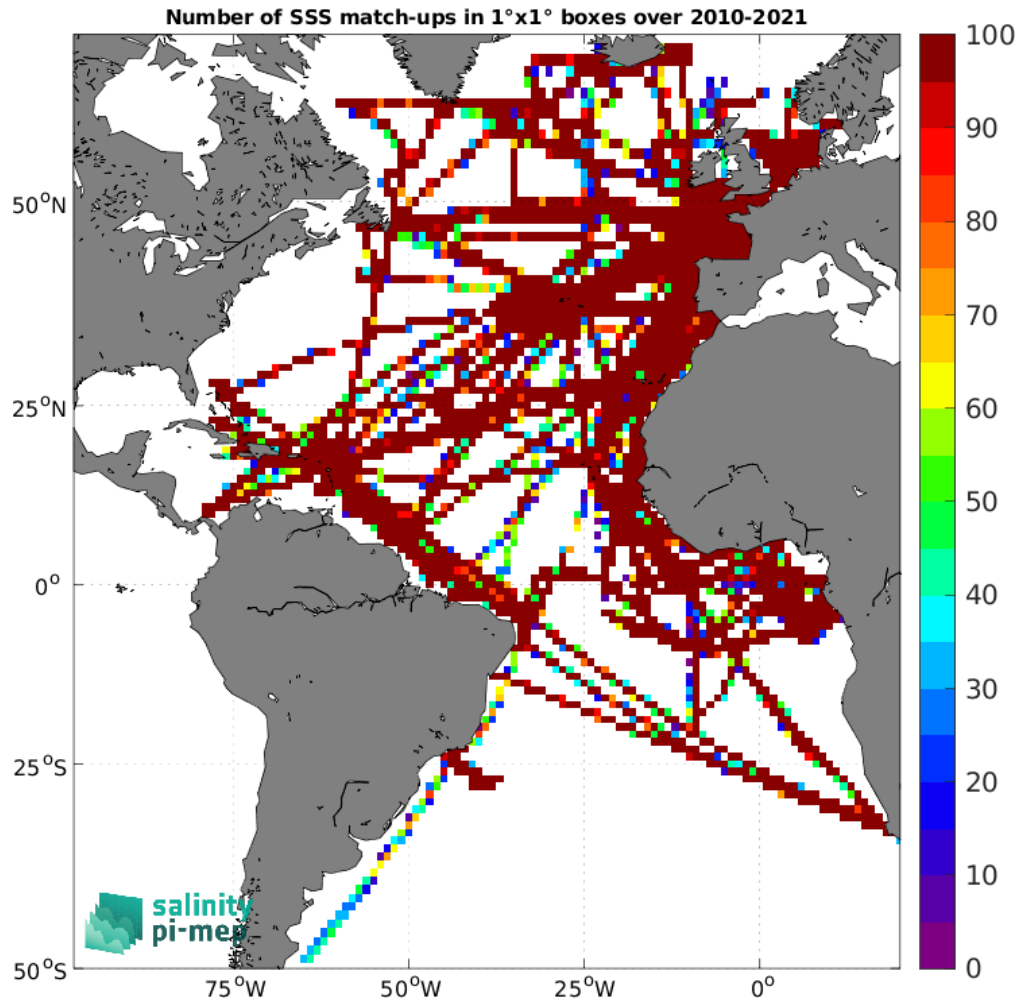
Figure 4: Number of SSS match-ups between TSG (GOSUD-Research-vessel) SSS and the SMOS SSS L4 v1 - Weekly (CMEMS-CNR) SSS product for the Atlantic Ocean Pi-MEP region over 1^\circ \times 1^\circ boxes and for the full satellite product period.
