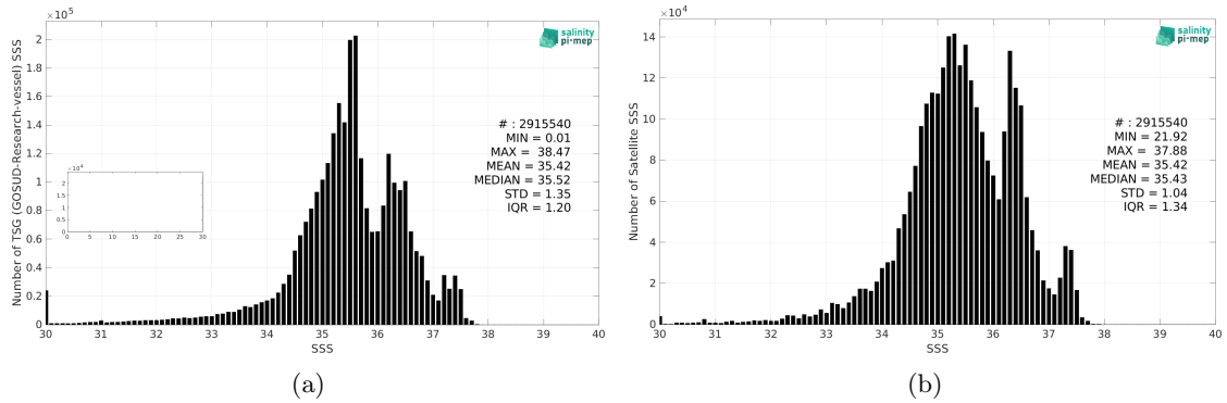
Figure 2: Histograms of SSS from TSG (GOSUD-Research-vessel) (a) and SMOS SSS L4 v1 - Weekly (CMEMS-CNR) (b) considering all match-up pairs per bins of 0.1 over the Atlantic Ocean Pi-MEP region and for the full satellite product period.
